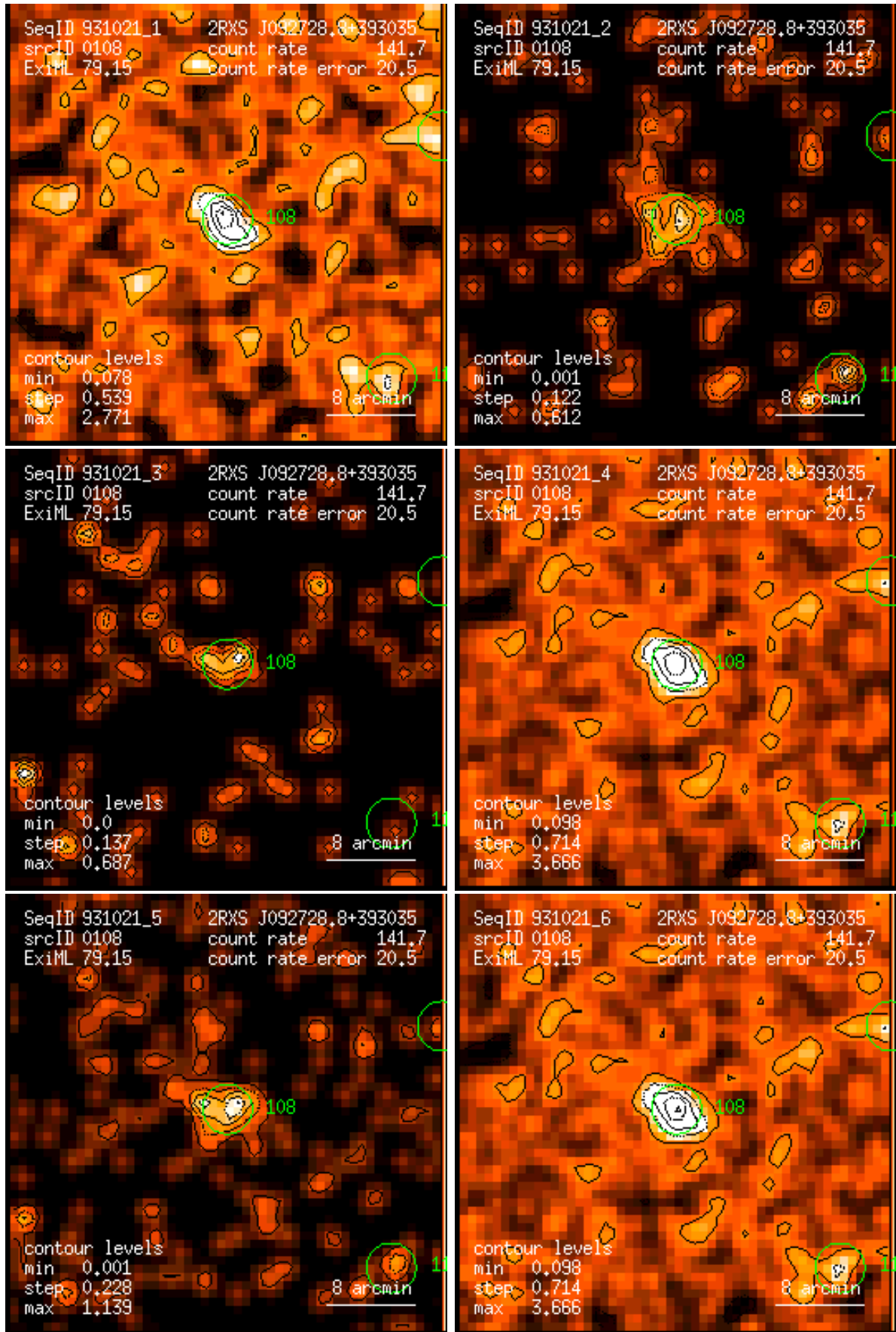
Figure 108: RASS 931021: detection 0108: band rate images, Gaussian filter: (1) PSPC channels 11 – 41, (2) 52 – 90, (3) 91 – 201, (4) 11 – 235, (5) 52 – 201, (6) 11 – 201. Broad band rates in counts/ks. Band rate contour levels in counts/ks/arcmin 2 .
