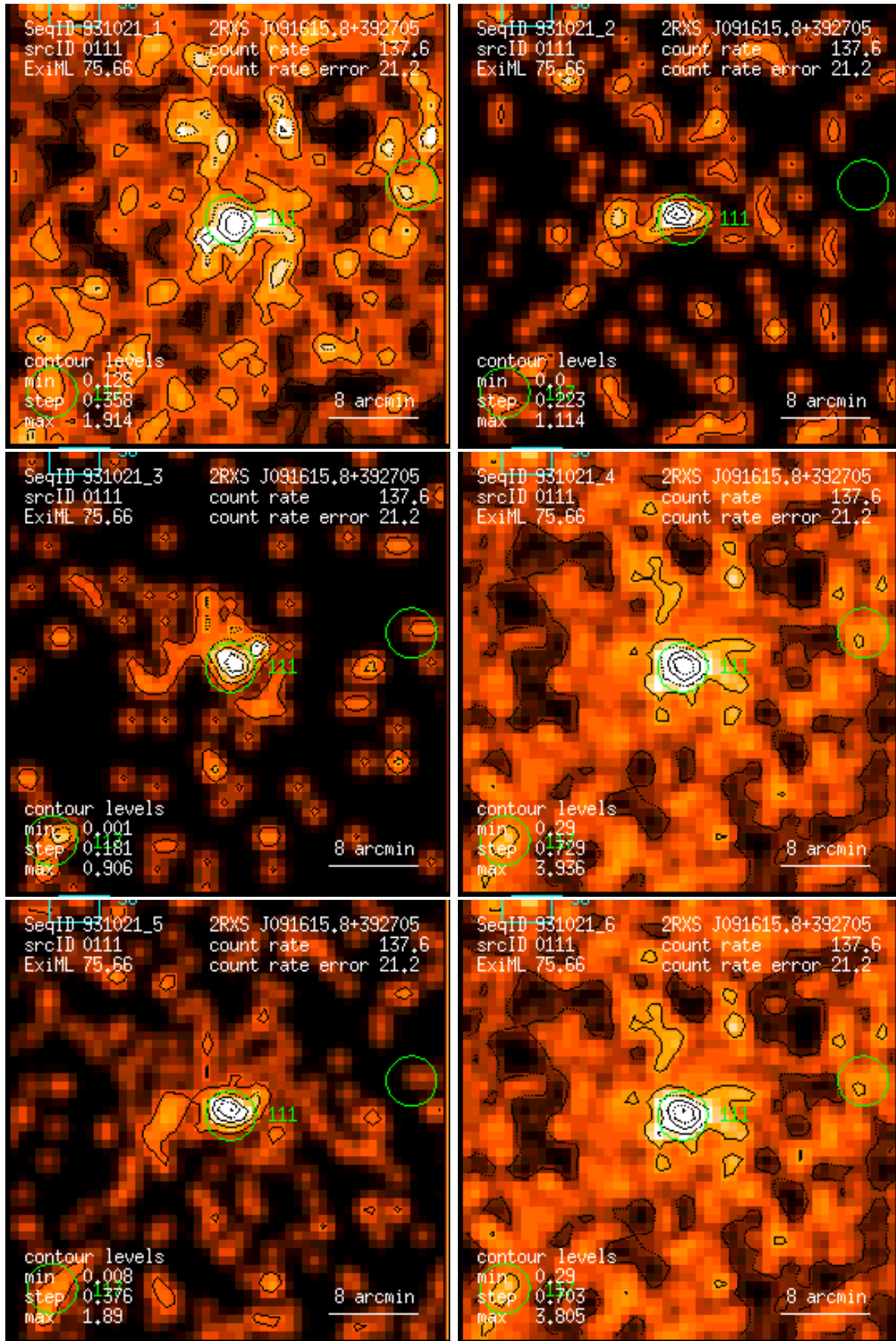
Figure 111: RASS 931021: detection 0111: band rate images, Gaussian filter: (1) PSPC channels 11 – 41, (2) 52 – 90, (3) 91 – 201, (4) 11 – 235, (5) 52 – 201, (6) 11 – 201. Broad band rates in counts/ks. Band rate contour levels in counts/ks/arcmin 2 .
