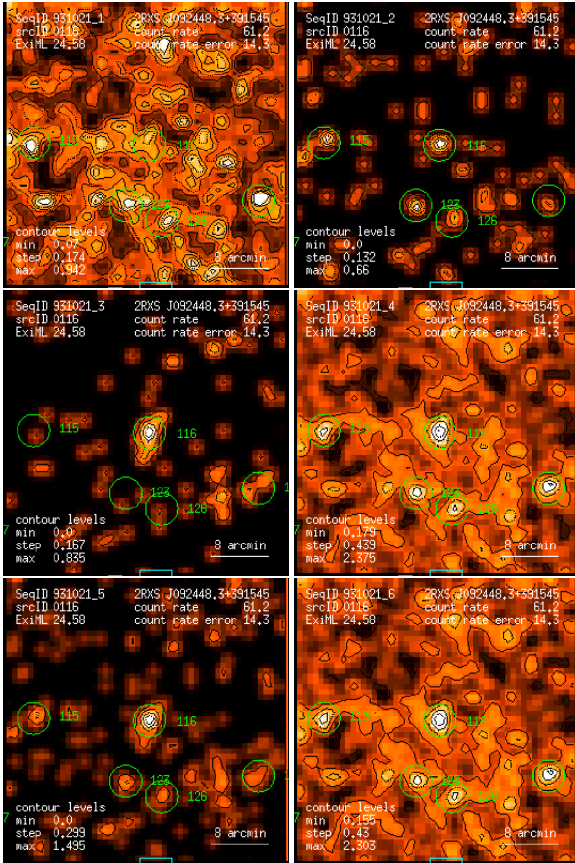
Figure 116: RASS 931021: detection 0116: band rate images, Gaussian filter: (1) PSPC channels 11 – 41, (2) 52 – 90, (3) 91 – 201, (4) 11 – 235, (5) 52 – 201, (6) 11 – 201. Broad band rates in counts/ks. Band rate contour levels in counts/ks/arcmin 2 .
