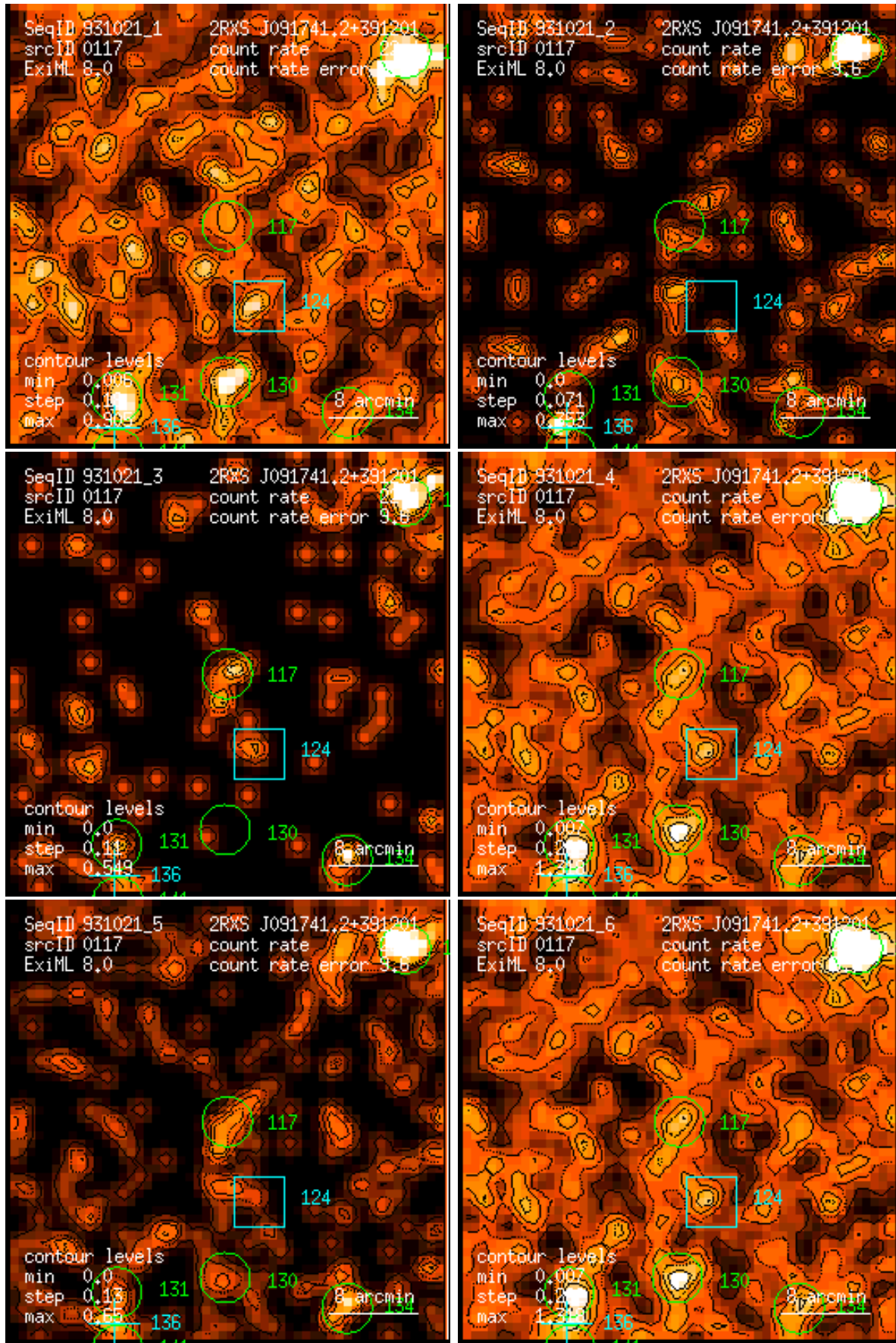
Figure 117: RASS 931021: detection 0117: band rate images, Gaussian filter: (1) PSPC channels 11 – 41, (2) 52 – 90, (3) 91 – 201, (4) 11 – 235, (5) 52 – 201, (6) 11 – 201. Broad band rates in counts/ks. Band rate contour levels in counts/ks/arcmin 2 .
