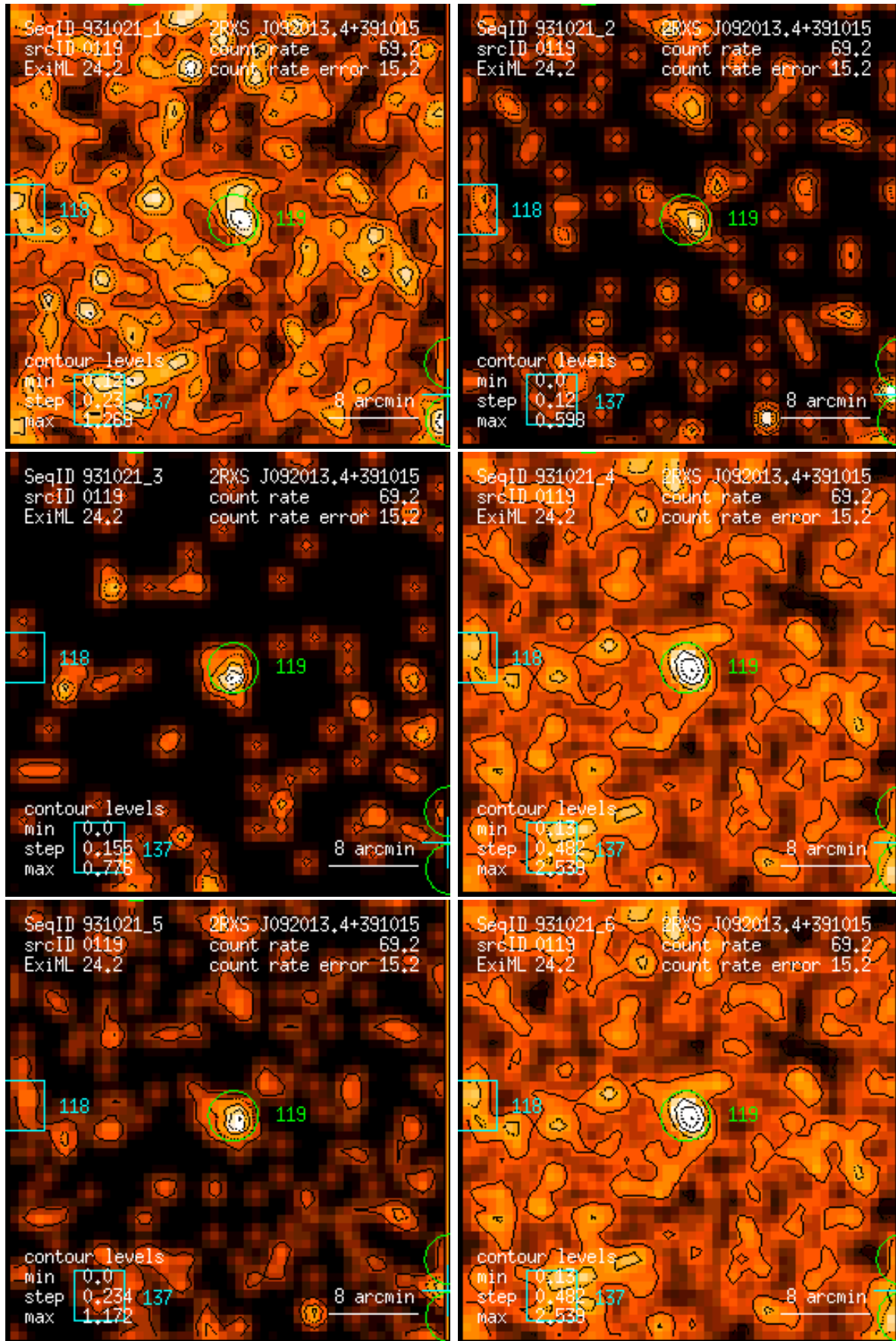
Figure 119: RASS 931021: detection 0119: band rate images, Gaussian filter: (1) PSPC channels 11 – 41, (2) 52 – 90, (3) 91 – 201, (4) 11 – 235, (5) 52 – 201, (6) 11 – 201. Broad band rates in counts/ks. Band rate contour levels in counts/ks/arcmin 2 .
