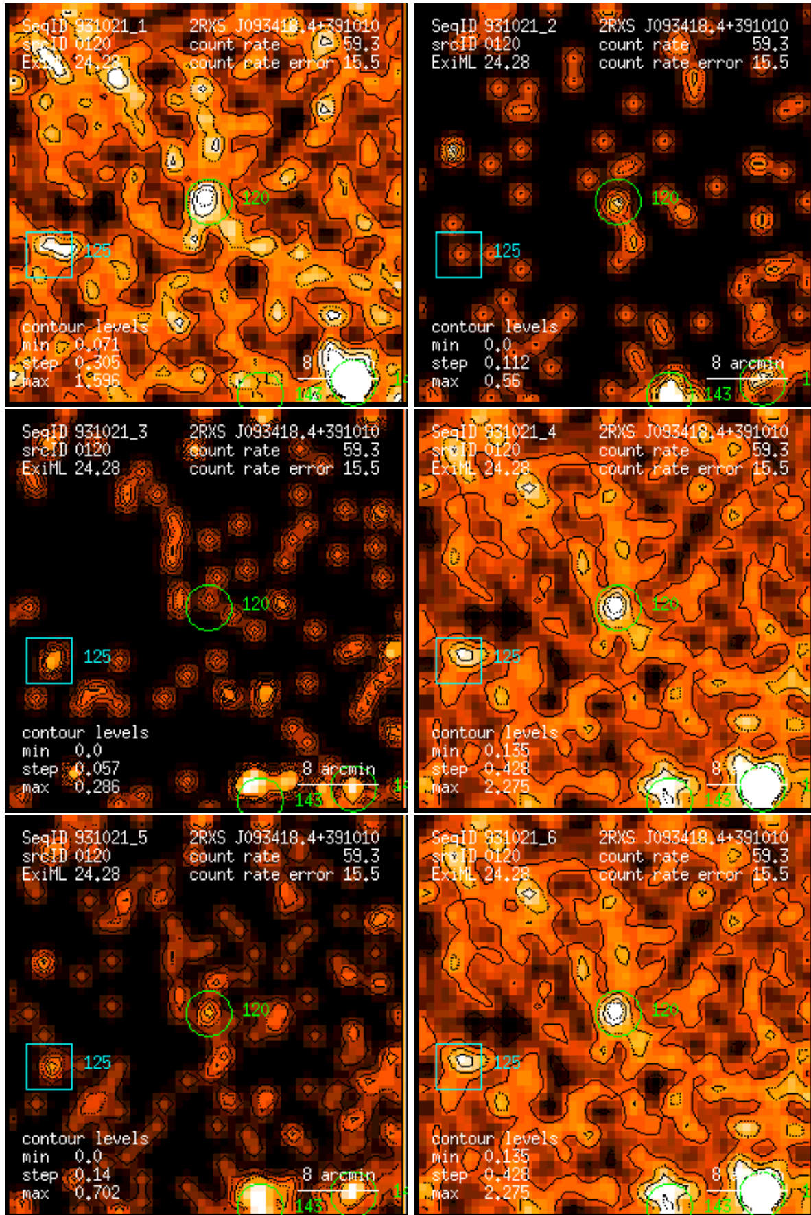
Figure 120: RASS 931021: detection 0120: band rate images, Gaussian filter: (1) PSPC channels 11 – 41, (2) 52 – 90, (3) 91 – 201, (4) 11 – 235, (5) 52 – 201, (6) 11 – 201. Broad band rates in counts/ks. Band rate contour levels in counts/ks/arcmin 2 .
