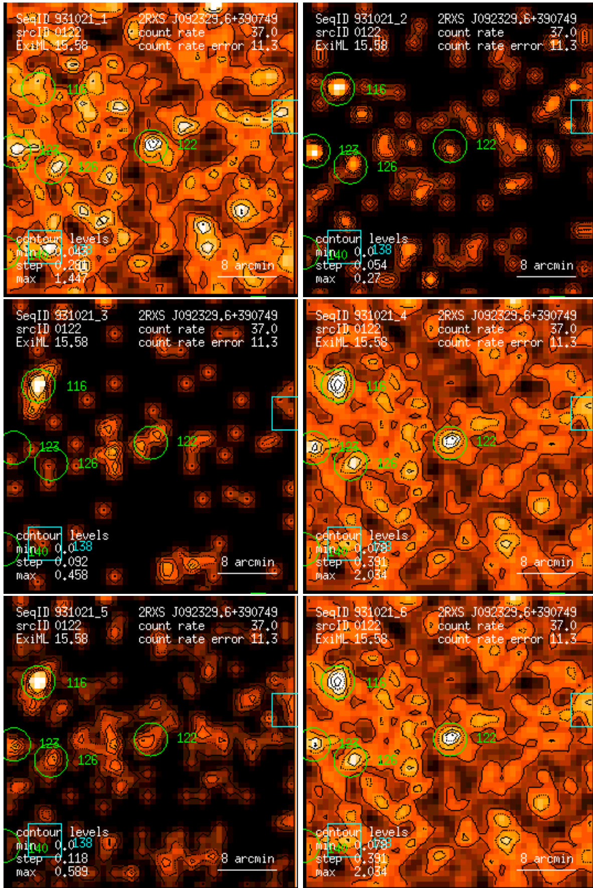
Figure 122: RASS 931021: detection 0122: band rate images, Gaussian filter: (1) PSPC channels 11 – 41, (2) 52 – 90, (3) 91 – 201, (4) 11 – 235, (5) 52 – 201, (6) 11 – 201. Broad band rates in counts/ks. Band rate contour levels in counts/ks/arcmin 2 .
