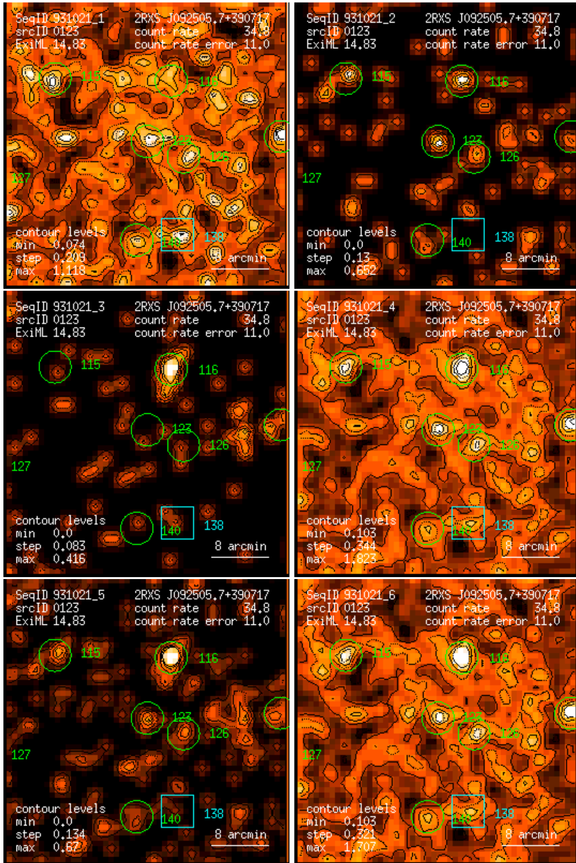
Figure 123: RASS 931021: detection 0123: band rate images, Gaussian filter: (1) PSPC channels 11 – 41, (2) 52 – 90, (3) 91 – 201, (4) 11 – 235, (5) 52 – 201, (6) 11 – 201. Broad band rates in counts/ks. Band rate contour levels in counts/ks/arcmin 2 .
