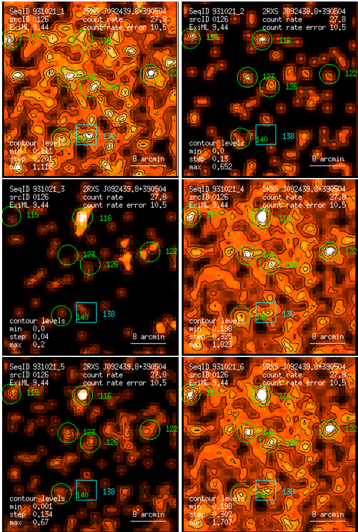
Figure 126: RASS 931021: detection 0126: band rate images, Gaussian filter: (1) PSPC channels 11 – 41, (2) 52 – 90, (3) 91 – 201, (4) 11 – 235, (5) 52 – 201, (6) 11 – 201. Broad band rates in counts/ks. Band rate contour levels in counts/ks/arcmin 2 .
