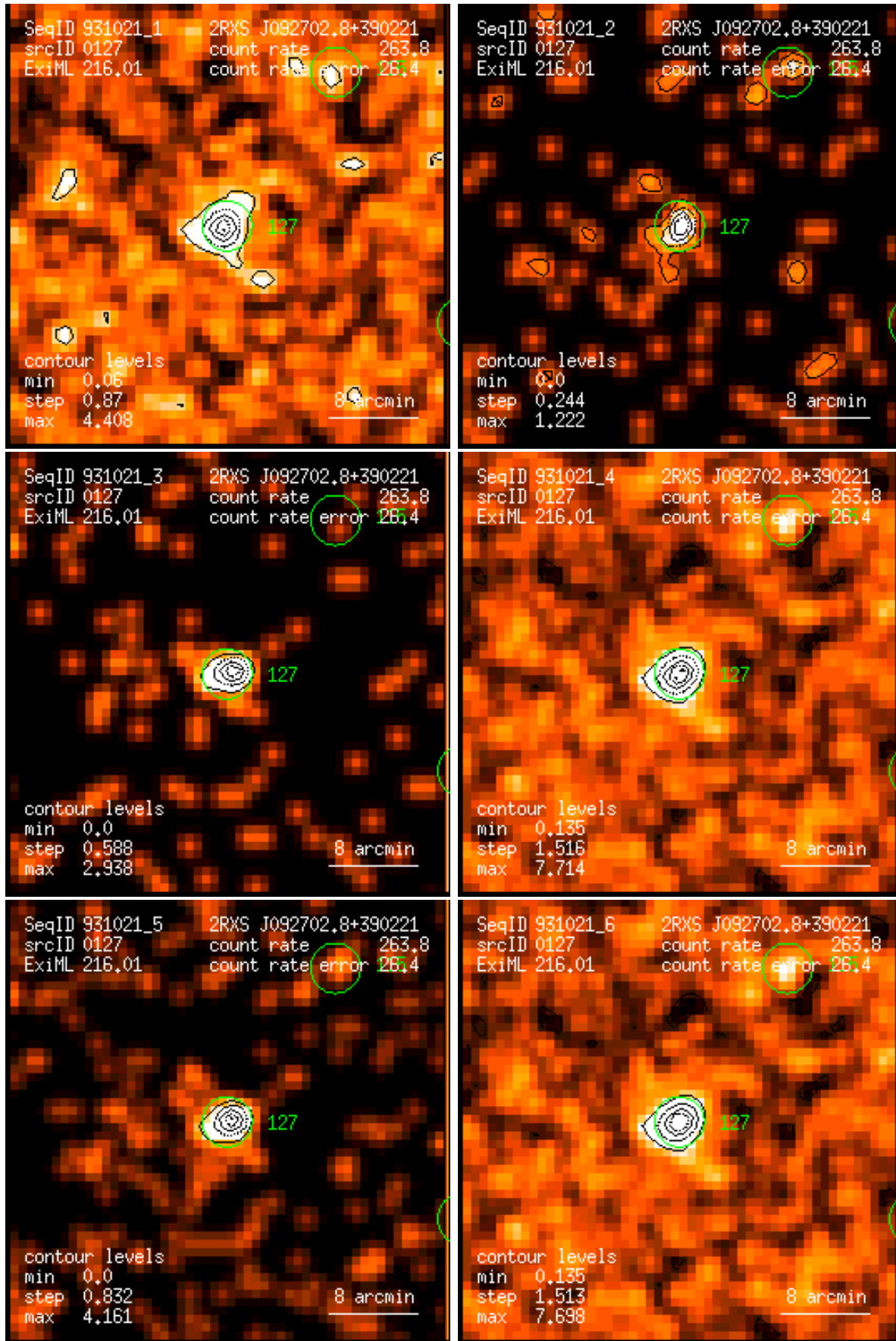
Figure 127: RASS 931021: detection 0127: band rate images, Gaussian filter: (1) PSPC channels 11 – 41, (2) 52 – 90, (3) 91 – 201, (4) 11 – 235, (5) 52 – 201, (6) 11 – 201. Broad band rates in counts/ks. Band rate contour levels in counts/ks/arcmin 2 .
