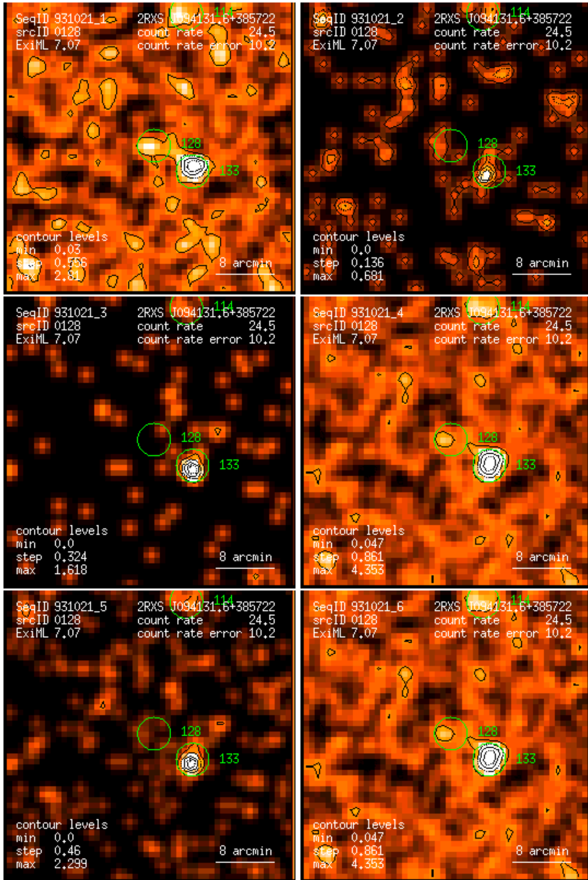
Figure 128: RASS 931021: detection 0128: band rate images, Gaussian filter: (1) PSPC channels 11 – 41, (2) 52 – 90, (3) 91 – 201, (4) 11 – 235, (5) 52 – 201, (6) 11 – 201. Broad band rates in counts/ks. Band rate contour levels in counts/ks/arcmin 2 .
