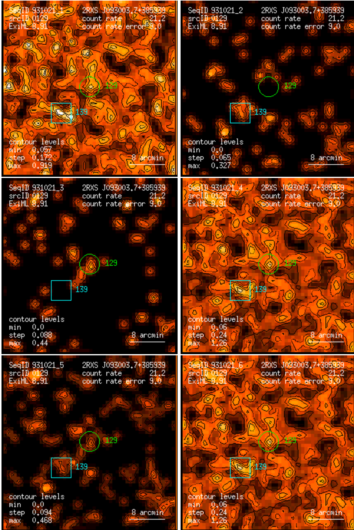
Figure 129: RASS 931021: detection 0129: band rate images, Gaussian filter: (1) PSPC channels 11 – 41, (2) 52 – 90, (3) 91 – 201, (4) 11 – 235, (5) 52 – 201, (6) 11 – 201. Broad band rates in counts/ks. Band rate contour levels in counts/ks/arcmin 2 .
