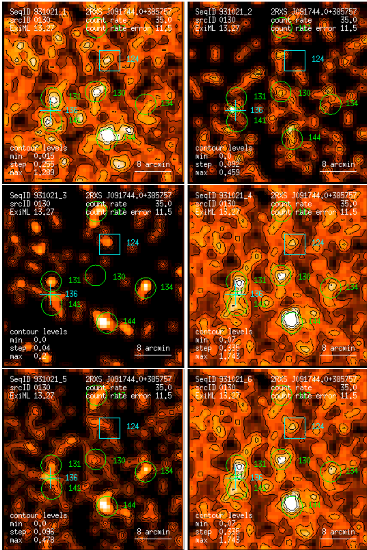
Figure 130: RASS 931021: detection 0130: band rate images, Gaussian filter: (1) PSPC channels 11 – 41, (2) 52 – 90, (3) 91 – 201, (4) 11 – 235, (5) 52 – 201, (6) 11 – 201. Broad band rates in counts/ks. Band rate contour levels in counts/ks/arcmin 2 .
