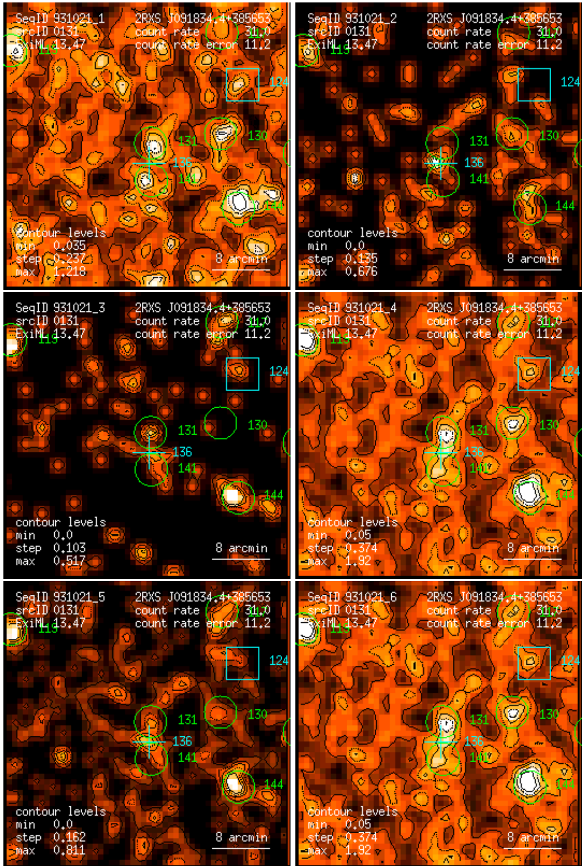
Figure 131: RASS 931021: detection 0131: band rate images, Gaussian filter: (1) PSPC channels 11 – 41, (2) 52 – 90, (3) 91 – 201, (4) 11 – 235, (5) 52 – 201, (6) 11 – 201. Broad band rates in counts/ks. Band rate contour levels in counts/ks/arcmin 2 .
