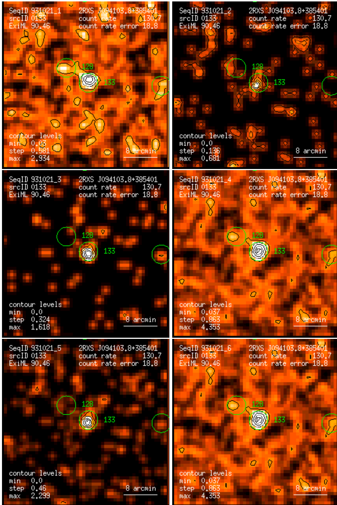
Figure 133: RASS 931021: detection 0133: band rate images, Gaussian filter: (1) PSPC channels 11 – 41, (2) 52 – 90, (3) 91 – 201, (4) 11 – 235, (5) 52 – 201, (6) 11 – 201. Broad band rates in counts/ks. Band rate contour levels in counts/ks/arcmin 2 .
