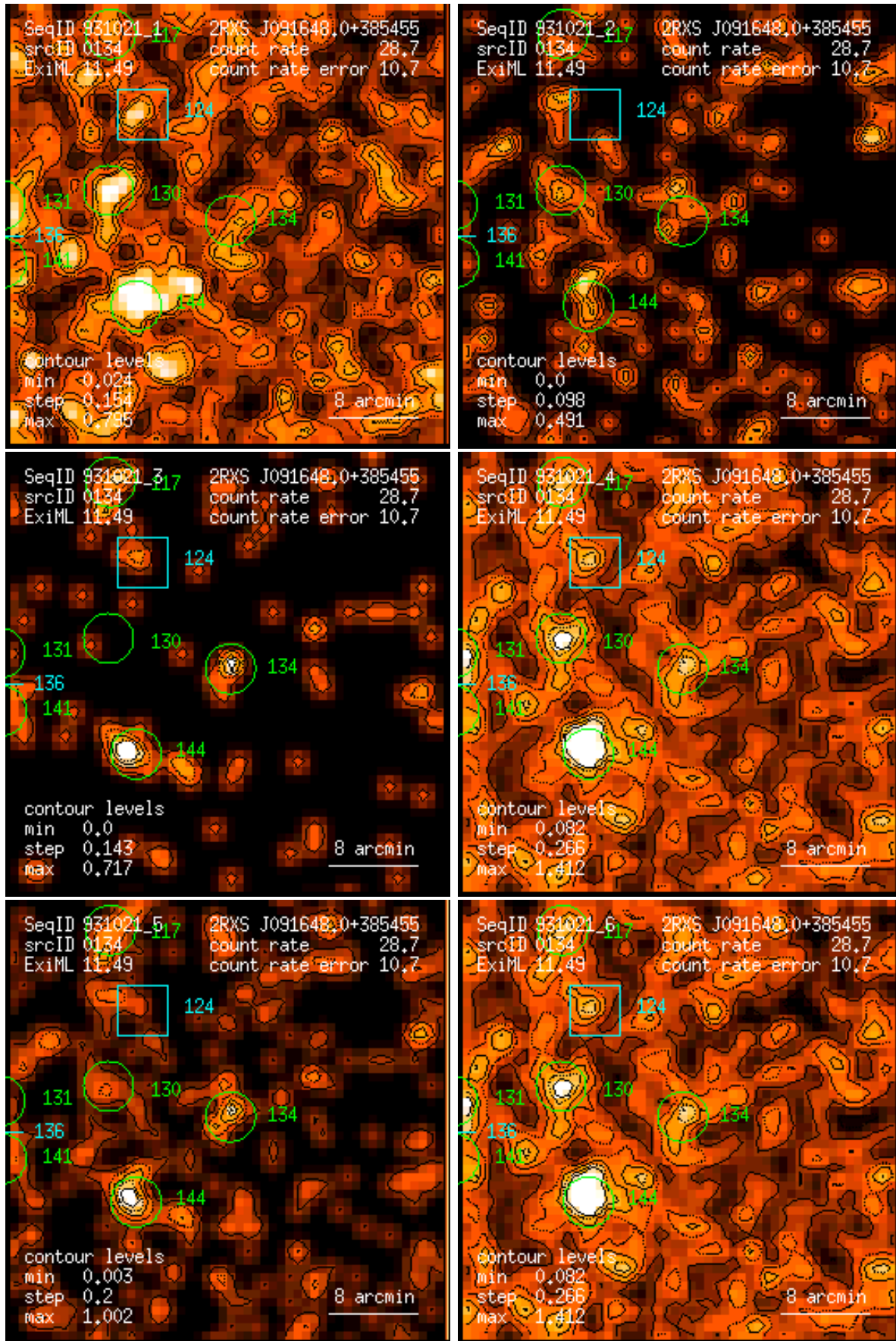
Figure 134: RASS 931021: detection 0134: band rate images, Gaussian filter: (1) PSPC channels 11 – 41, (2) 52 – 90, (3) 91 – 201, (4) 11 – 235, (5) 52 – 201, (6) 11 – 201. Broad band rates in counts/ks. Band rate contour levels in counts/ks/arcmin 2 .
