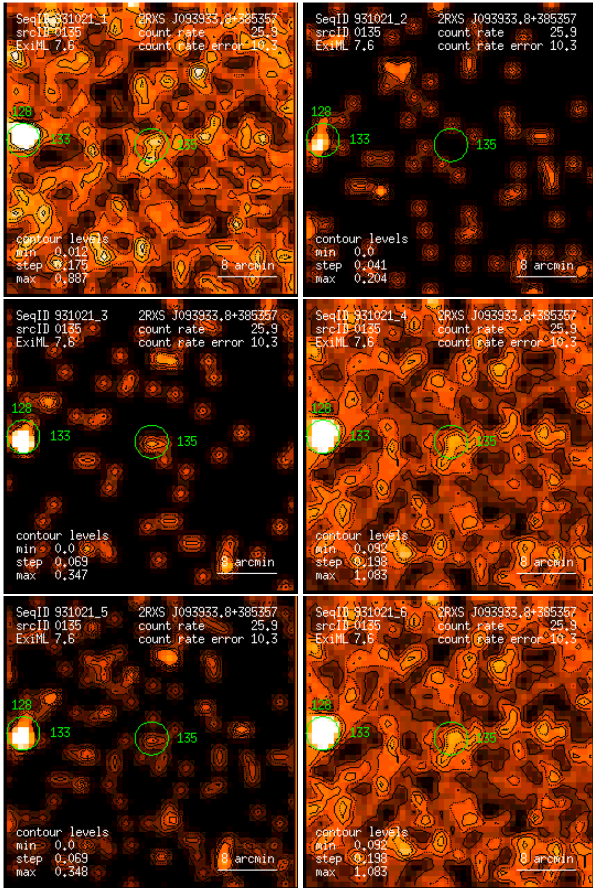
Figure 135: RASS 931021: detection 0135: band rate images, Gaussian filter: (1) PSPC channels 11 – 41, (2) 52 – 90, (3) 91 – 201, (4) 11 – 235, (5) 52 – 201, (6) 11 – 201. Broad band rates in counts/ks. Band rate contour levels in counts/ks/arcmin 2 .
