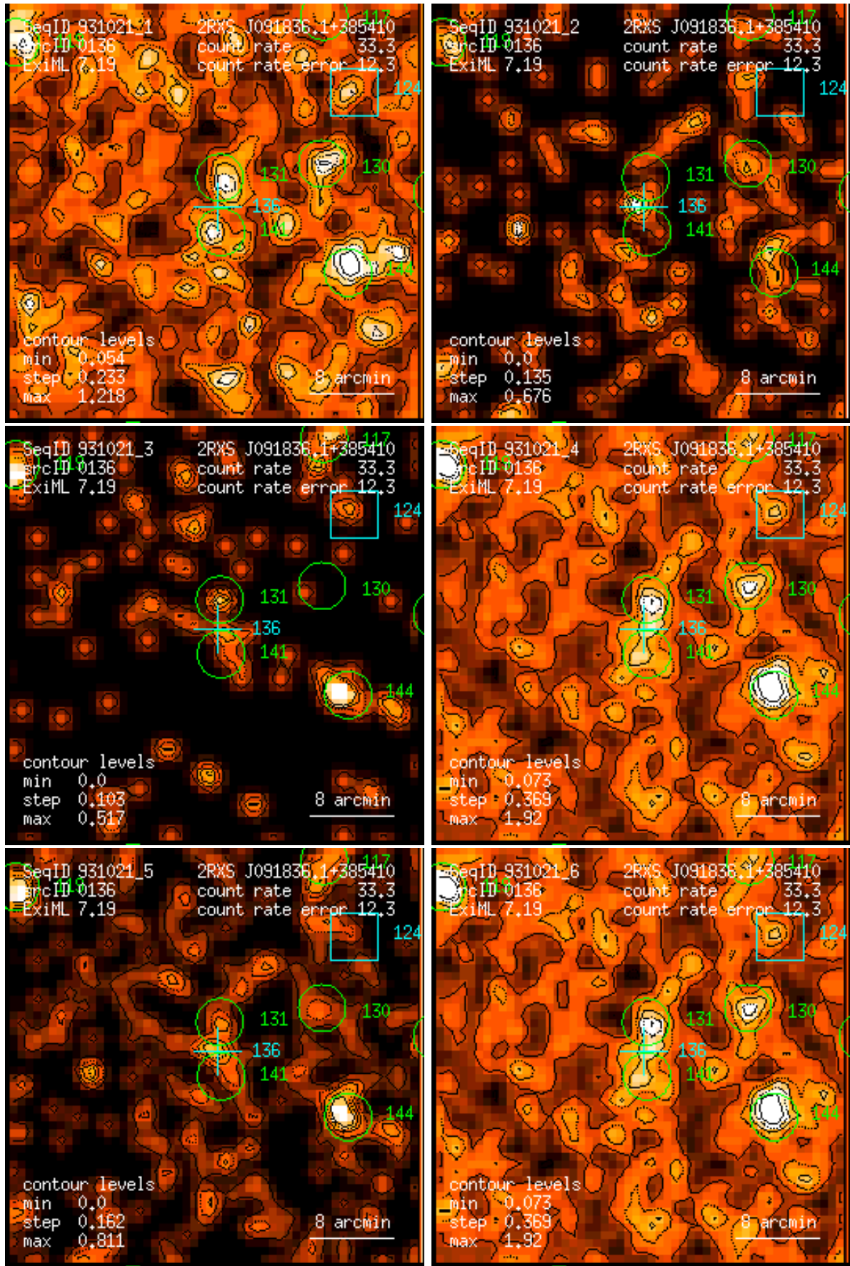
Figure 136: RASS 931021: detection 0136: band rate images, Gaussian filter: (1) PSPC channels 11 – 41, (2) 52 – 90, (3) 91 – 201, (4) 11 – 235, (5) 52 – 201, (6) 11 – 201. Broad band rates in counts/ks. Band rate contour levels in counts/ks/arcmin 2 .
