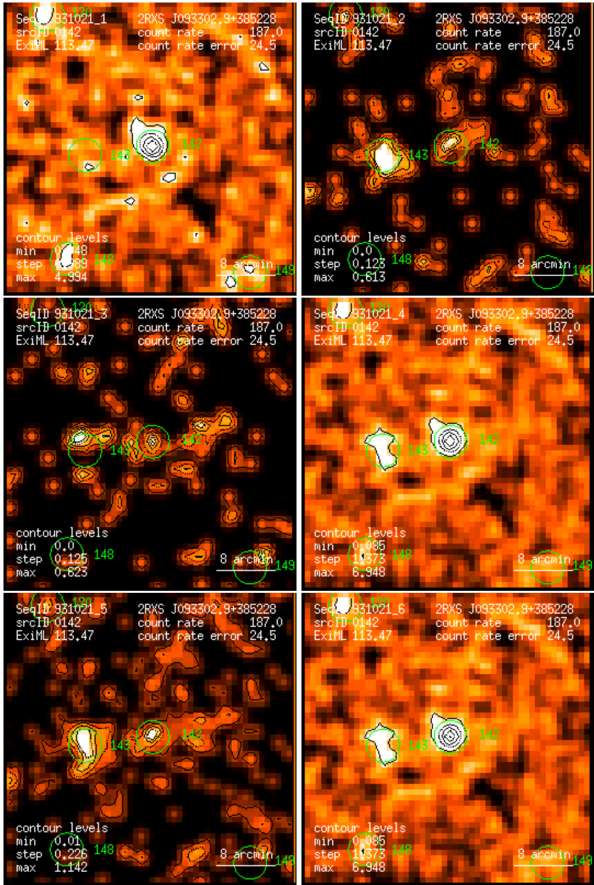
Figure 142: RASS 931021: detection 0142: band rate images, Gaussian filter: (1) PSPC channels 11 – 41, (2) 52 – 90, (3) 91 – 201, (4) 11 – 235, (5) 52 – 201, (6) 11 – 201. Broad band rates in counts/ks. Band rate contour levels in counts/ks/arcmin 2 .
