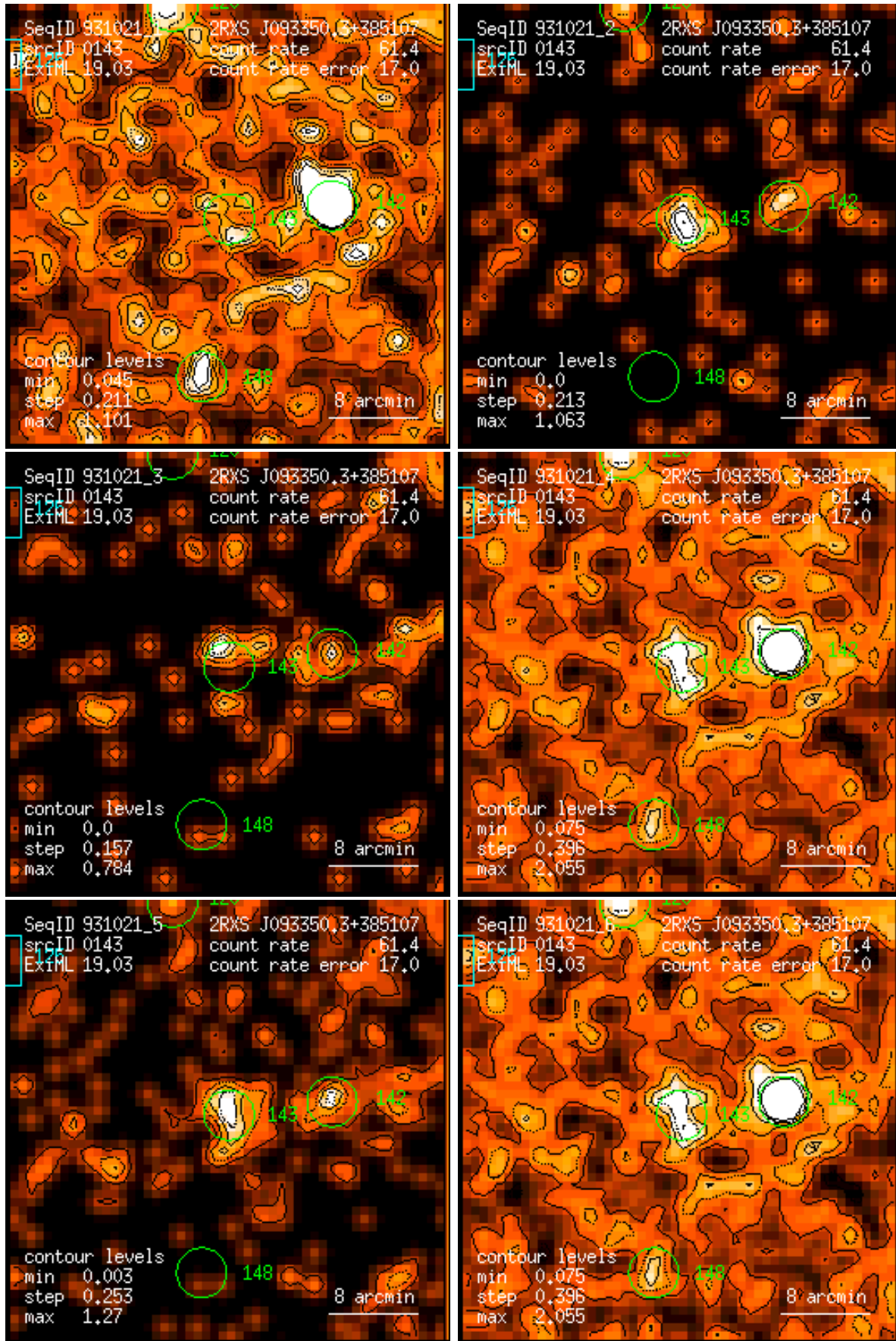
Figure 143: RASS 931021: detection 0143: band rate images, Gaussian filter: (1) PSPC channels 11 – 41, (2) 52 – 90, (3) 91 – 201, (4) 11 – 235, (5) 52 – 201, (6) 11 – 201. Broad band rates in counts/ks. Band rate contour levels in counts/ks/arcmin 2 .
