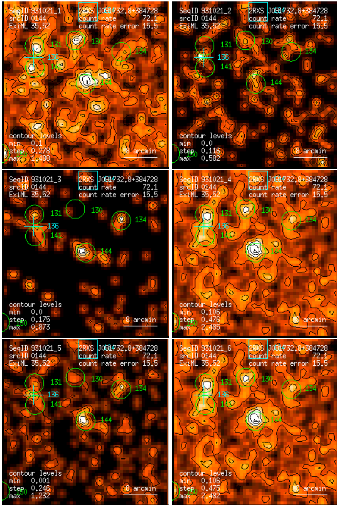
Figure 144: RASS 931021: detection 0144: band rate images, Gaussian filter: (1) PSPC channels 11 – 41, (2) 52 – 90, (3) 91 – 201, (4) 11 – 235, (5) 52 – 201, (6) 11 – 201. Broad band rates in counts/ks. Band rate contour levels in counts/ks/arcmin 2 .
