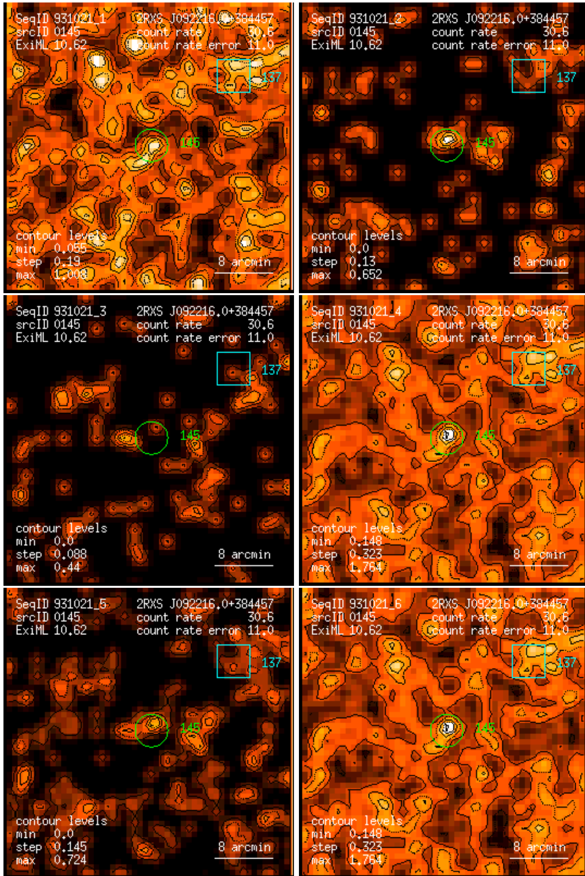
Figure 145: RASS 931021: detection 0145: band rate images, Gaussian filter: (1) PSPC channels 11 – 41, (2) 52 – 90, (3) 91 – 201, (4) 11 – 235, (5) 52 – 201, (6) 11 – 201. Broad band rates in counts/ks. Band rate contour levels in counts/ks/arcmin 2 .
