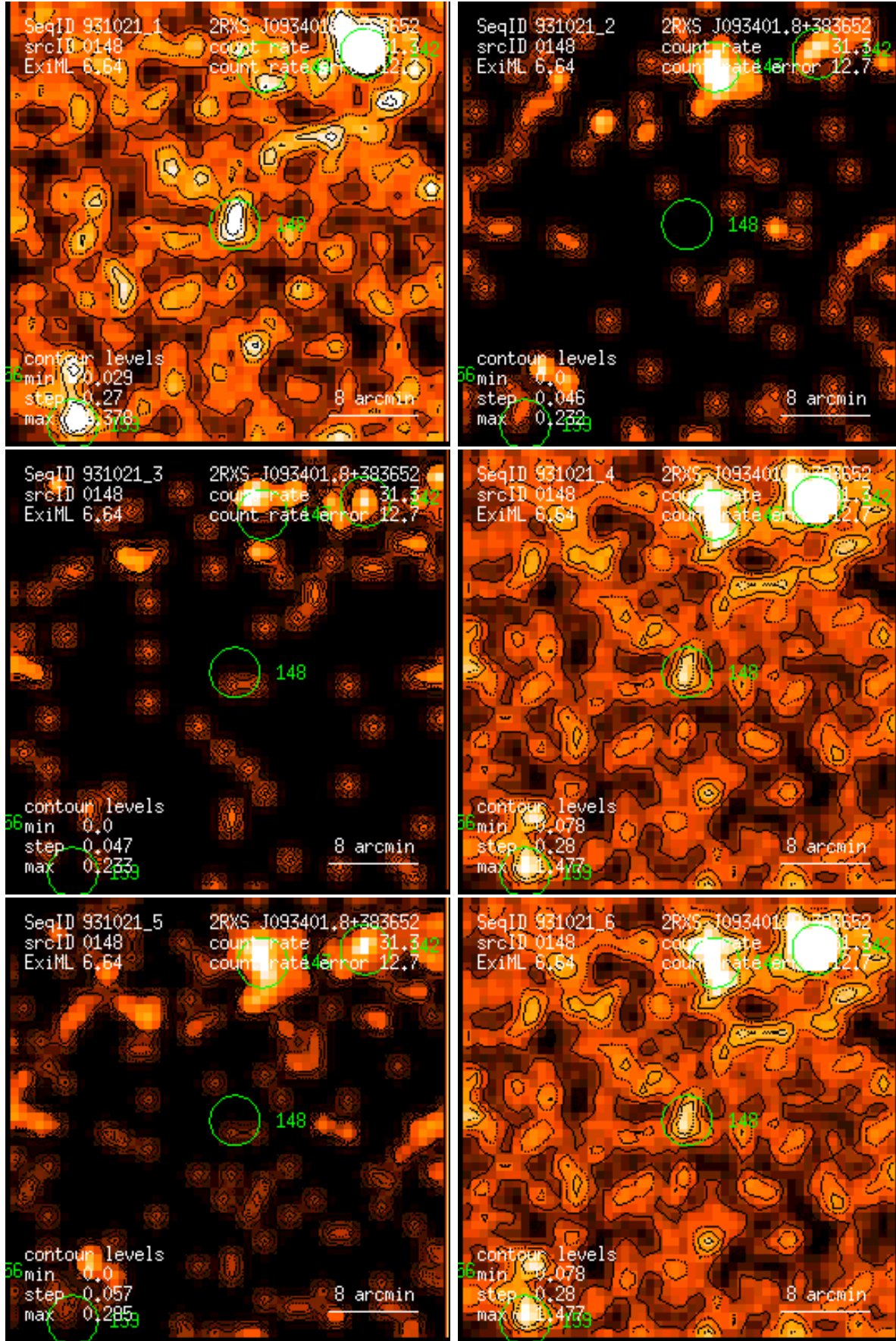
Figure 148: RASS 931021: detection 0148: band rate images, Gaussian filter: (1) PSPC channels 11 – 41, (2) 52 – 90, (3) 91 – 201, (4) 11 – 235, (5) 52 – 201, (6) 11 – 201. Broad band rates in counts/ks. Band rate contour levels in counts/ks/arcmin 2 .
