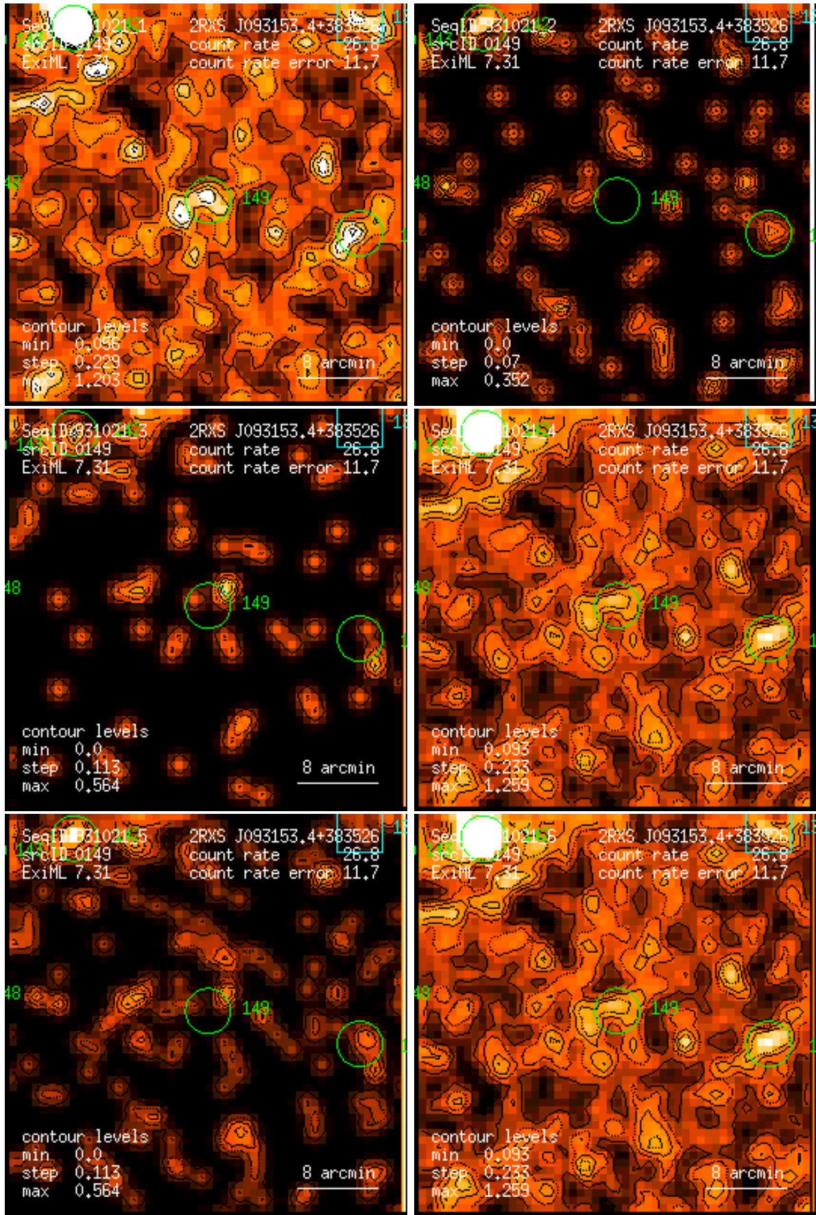
Figure 149: RASS 931021: detection 0149: band rate images, Gaussian filter: (1) PSPC channels 11 – 41, (2) 52 – 90, (3) 91 – 201, (4) 11 – 235, (5) 52 – 201, (6) 11 – 201. Broad band rates in counts/ks. Band rate contour levels in counts/ks/arcmin 2 .
