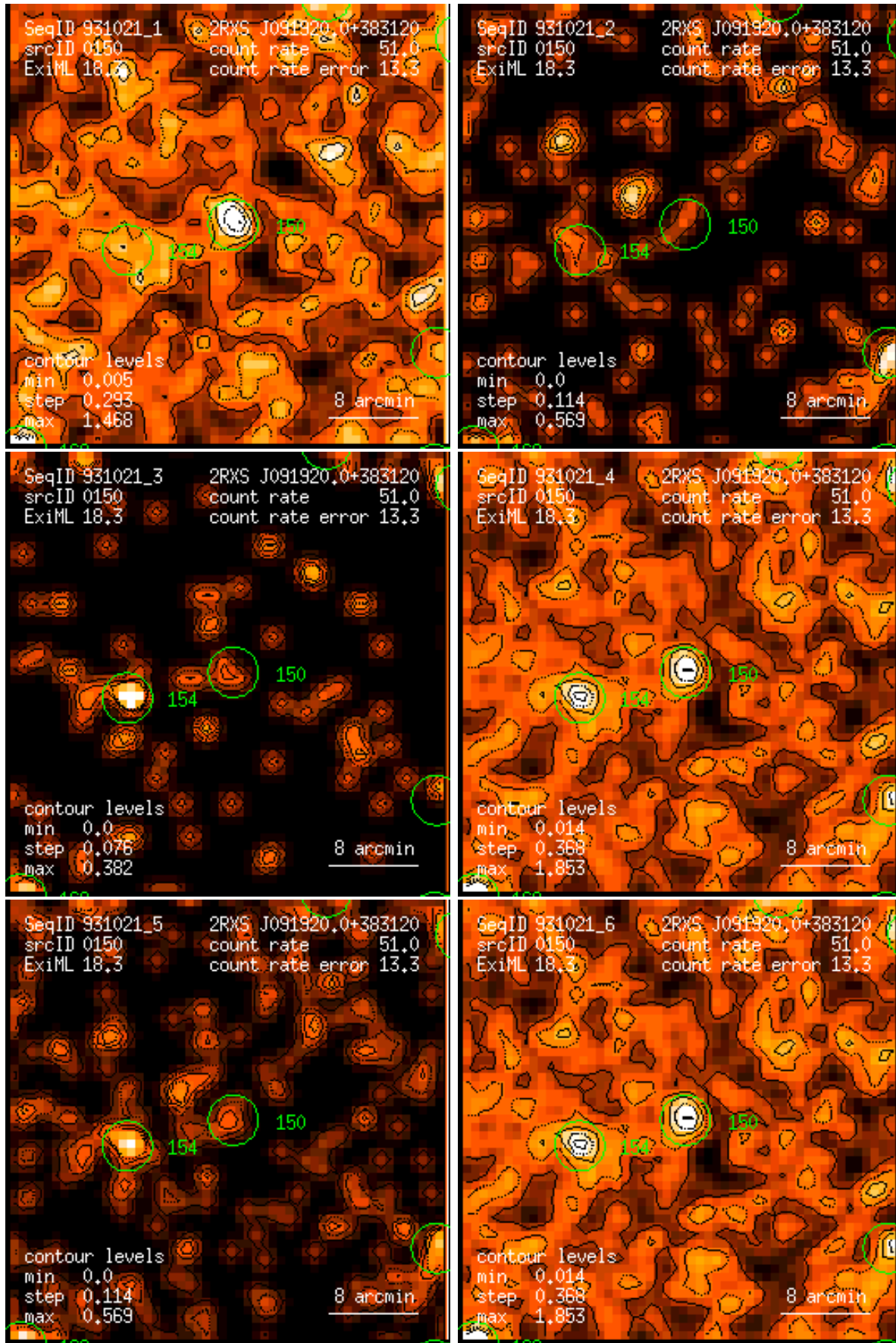
Figure 150: RASS 931021: detection 0150: band rate images, Gaussian filter: (1) PSPC channels 11 – 41, (2) 52 – 90, (3) 91 – 201, (4) 11 – 235, (5) 52 – 201, (6) 11 – 201. Broad band rates in counts/ks. Band rate contour levels in counts/ks/arcmin 2 .
