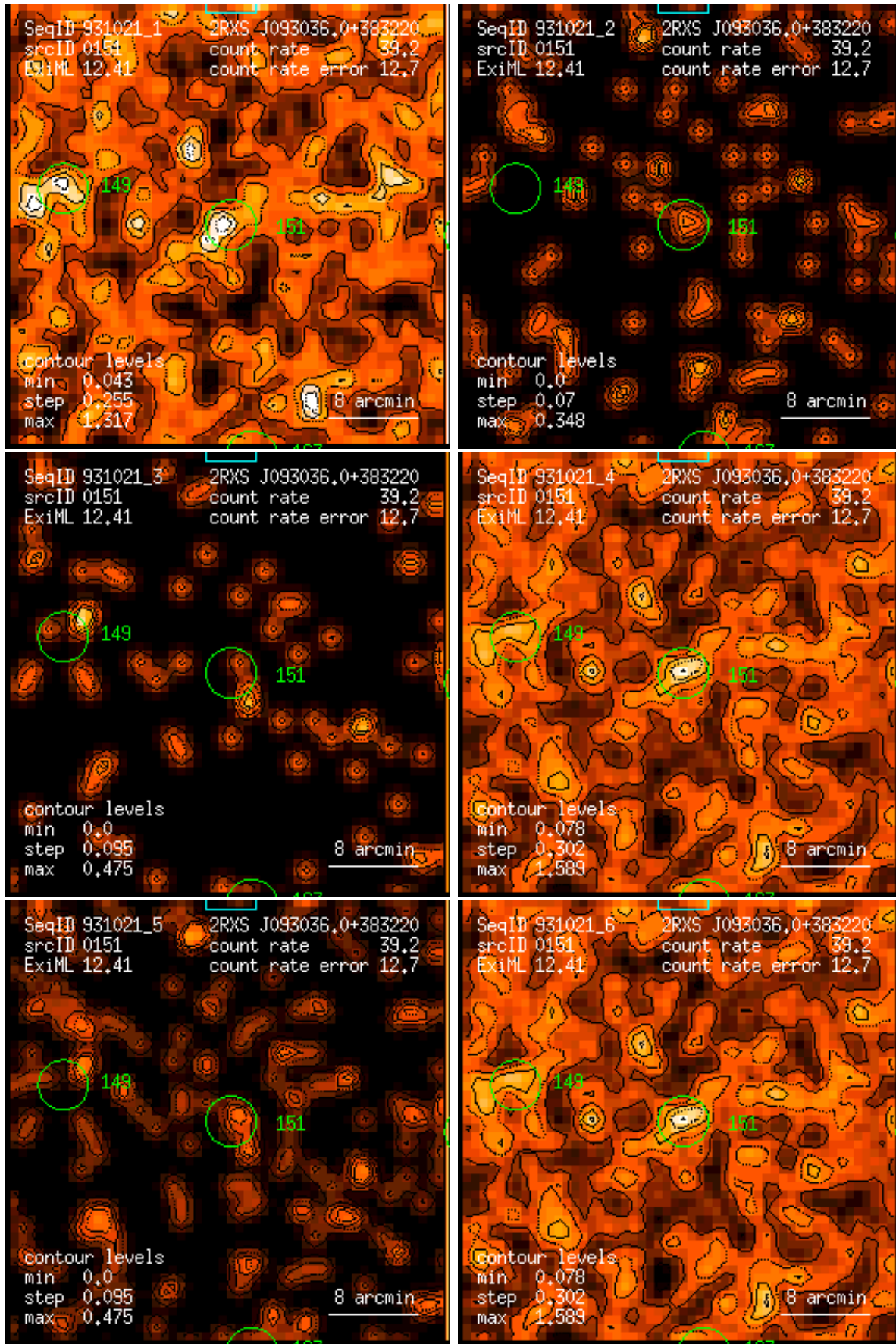
Figure 151: RASS 931021: detection 0151: band rate images, Gaussian filter: (1) PSPC channels 11 – 41, (2) 52 – 90, (3) 91 – 201, (4) 11 – 235, (5) 52 – 201, (6) 11 – 201. Broad band rates in counts/ks. Band rate contour levels in counts/ks/arcmin 2 .
