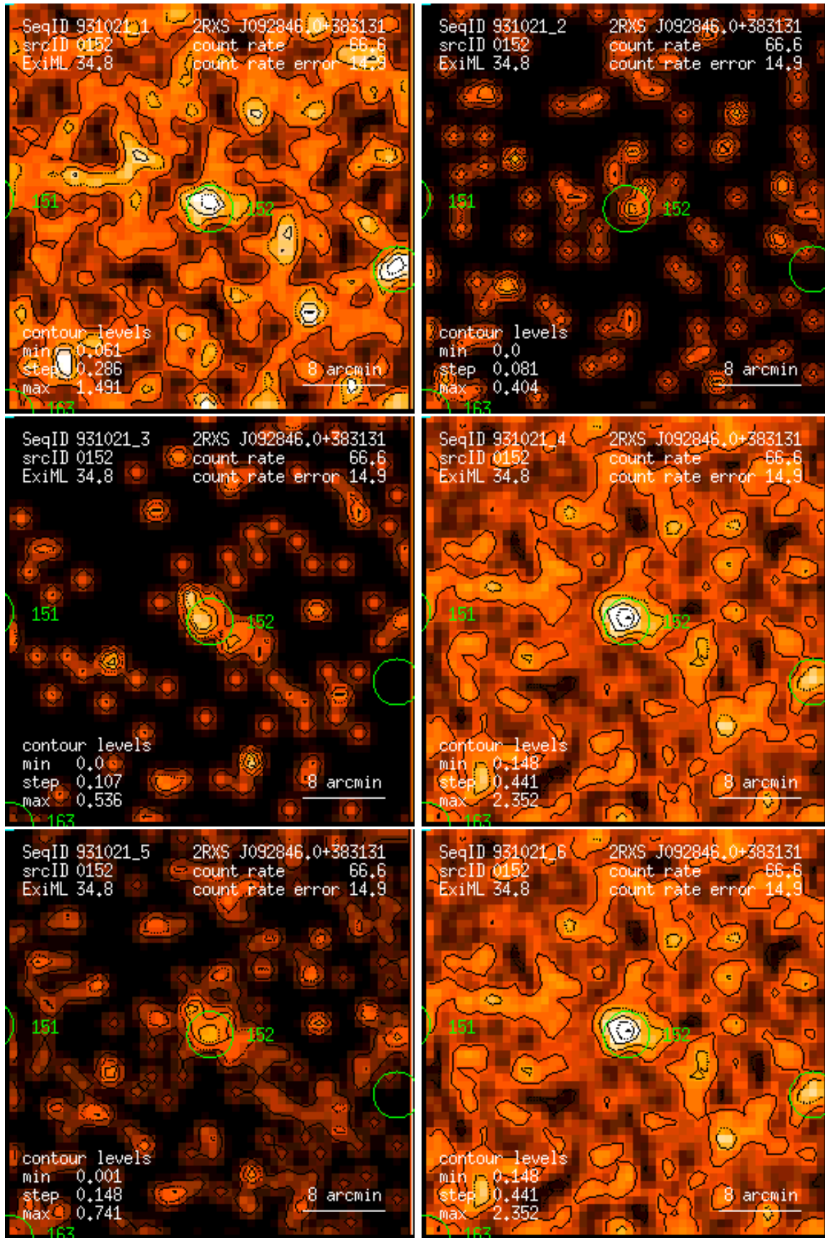
Figure 152: RASS 931021: detection 0152: band rate images, Gaussian filter: (1) PSPC channels 11 – 41, (2) 52 – 90, (3) 91 – 201, (4) 11 – 235, (5) 52 – 201, (6) 11 – 201. Broad band rates in counts/ks. Band rate contour levels in counts/ks/arcmin 2 .
