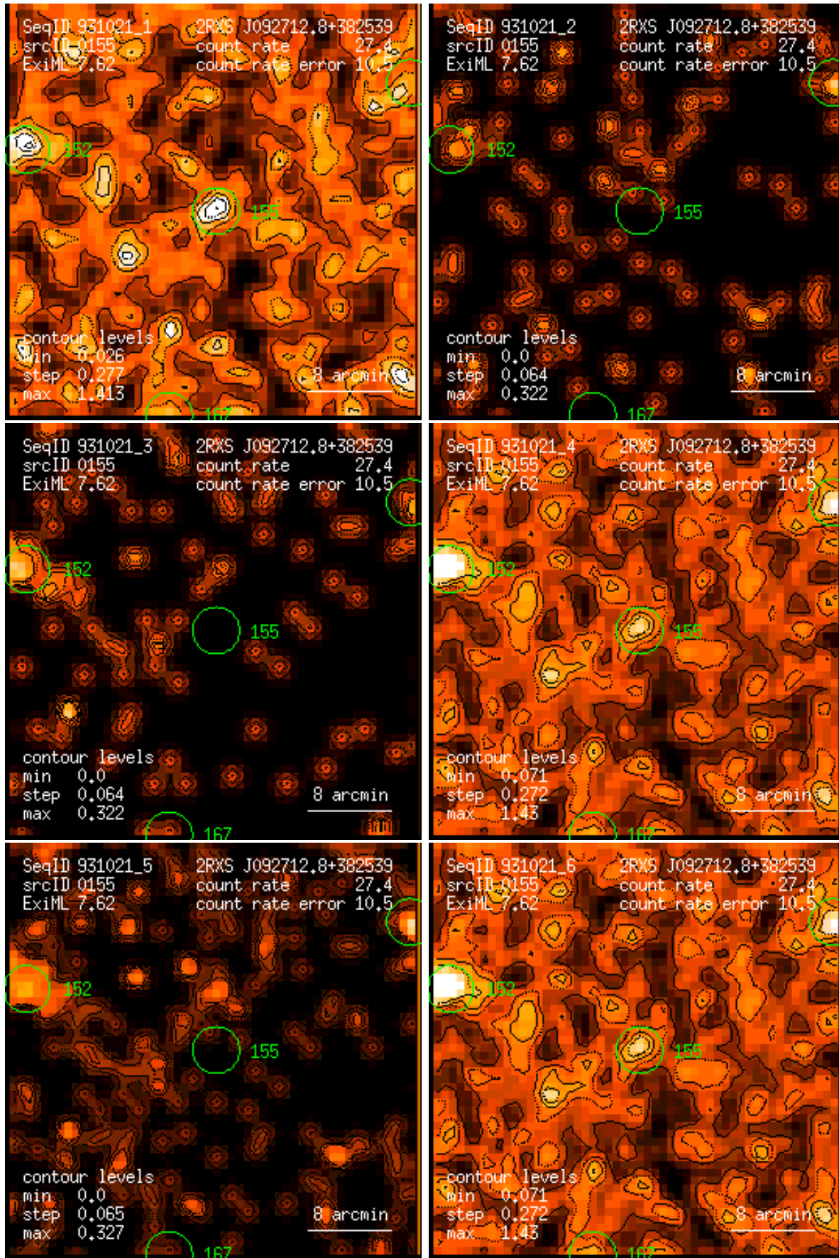
Figure 155: RASS 931021: detection 0155: band rate images, Gaussian filter: (1) PSPC channels 11 – 41, (2) 52 – 90, (3) 91 – 201, (4) 11 – 235, (5) 52 – 201, (6) 11 – 201. Broad band rates in counts/ks. Band rate contour levels in counts/ks/arcmin 2 .
