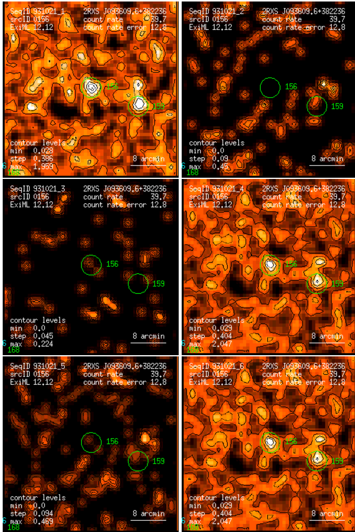
Figure 156: RASS 931021: detection 0156: band rate images, Gaussian filter: (1) PSPC channels 11 – 41, (2) 52 – 90, (3) 91 – 201, (4) 11 – 235, (5) 52 – 201, (6) 11 – 201. Broad band rates in counts/ks. Band rate contour levels in counts/ks/arcmin 2 .
