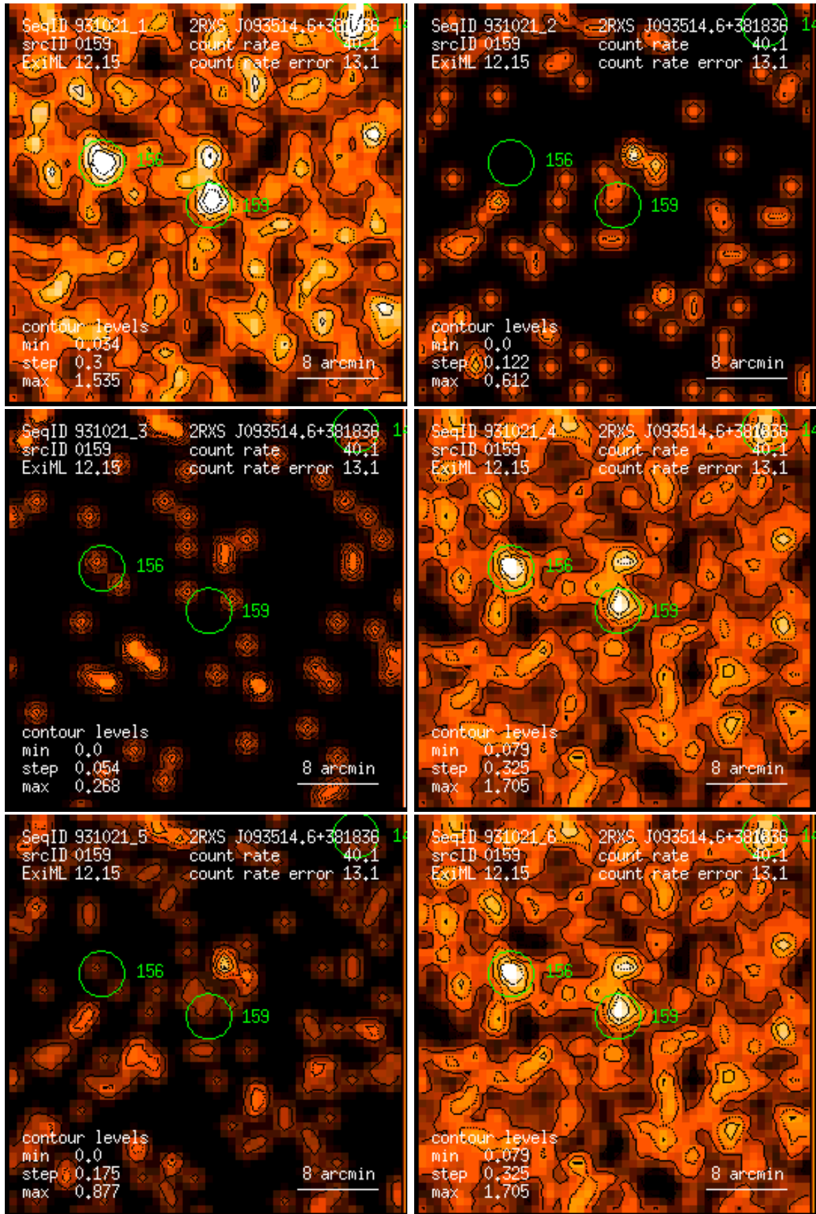
Figure 159: RASS 931021: detection 0159: band rate images, Gaussian filter: (1) PSPC channels 11 – 41, (2) 52 – 90, (3) 91 – 201, (4) 11 – 235, (5) 52 – 201, (6) 11 – 201. Broad band rates in counts/ks. Band rate contour levels in counts/ks/arcmin 2 .
