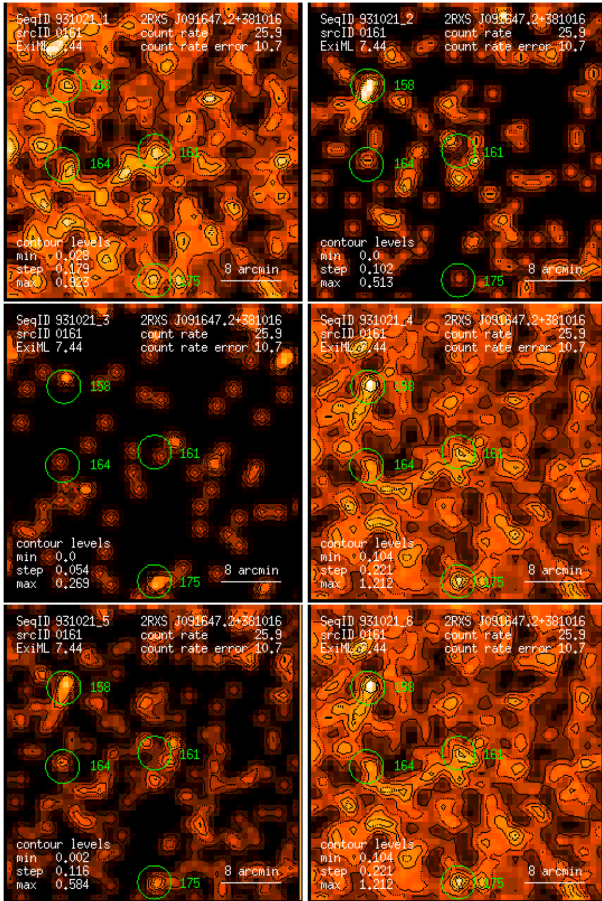
Figure 161: RASS 931021: detection 0161: band rate images, Gaussian filter: (1) PSPC channels 11 – 41, (2) 52 – 90, (3) 91 – 201, (4) 11 – 235, (5) 52 – 201, (6) 11 – 201. Broad band rates in counts/ks. Band rate contour levels in counts/ks/arcmin 2 .
