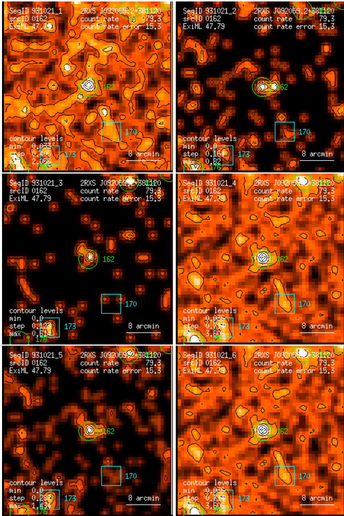
Figure 162: RASS 931021: detection 0162: band rate images, Gaussian filter: (1) PSPC channels 11 – 41, (2) 52 – 90, (3) 91 – 201, (4) 11 – 235, (5) 52 – 201, (6) 11 – 201. Broad band rates in counts/ks. Band rate contour levels in counts/ks/arcmin 2 .
