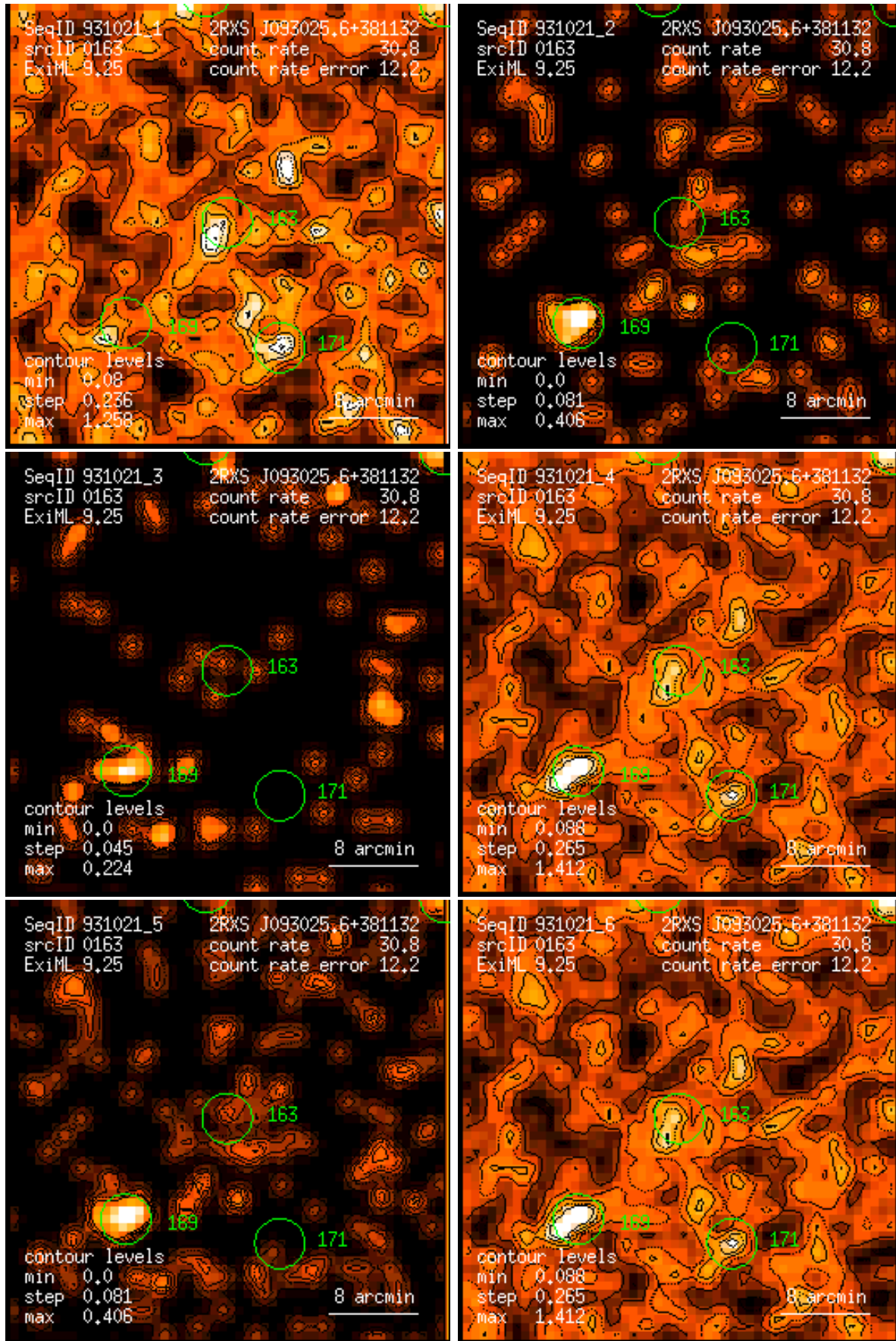
Figure 163: RASS 931021: detection 0163: band rate images, Gaussian filter: (1) PSPC channels 11 – 41, (2) 52 – 90, (3) 91 – 201, (4) 11 – 235, (5) 52 – 201, (6) 11 – 201. Broad band rates in counts/ks. Band rate contour levels in counts/ks/arcmin 2 .
