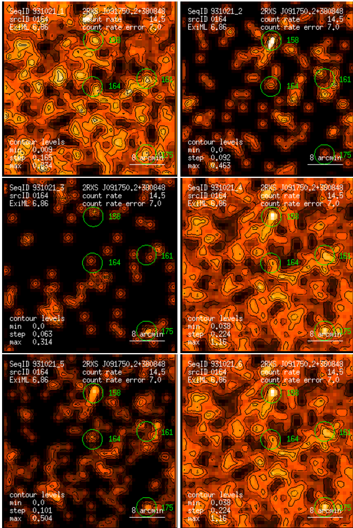
Figure 164: RASS 931021: detection 0164: band rate images, Gaussian filter: (1) PSPC channels 11 – 41, (2) 52 – 90, (3) 91 – 201, (4) 11 – 235, (5) 52 – 201, (6) 11 – 201. Broad band rates in counts/ks. Band rate contour levels in counts/ks/arcmin 2 .
