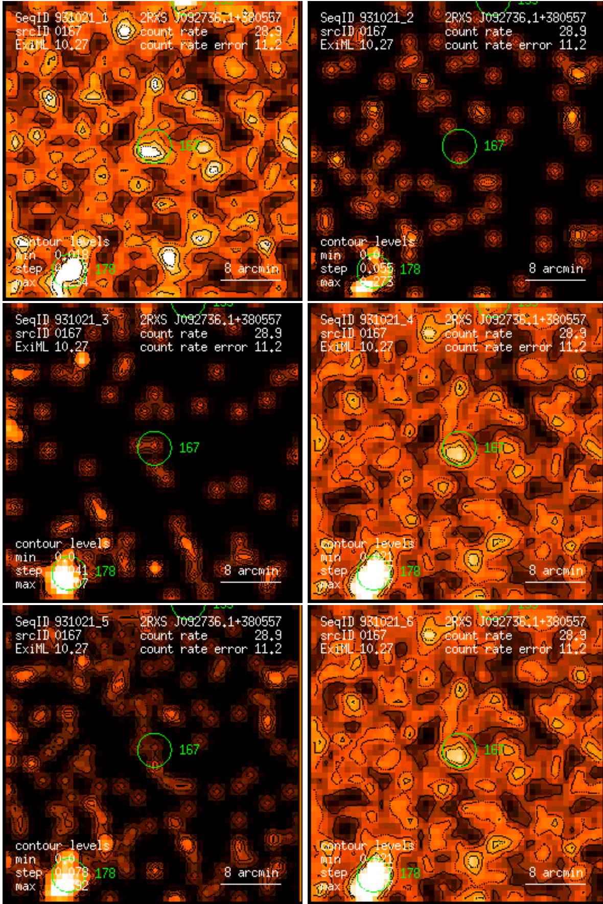
Figure 167: RASS 931021: detection 0167: band rate images, Gaussian filter: (1) PSPC channels 11 – 41, (2) 52 – 90, (3) 91 – 201, (4) 11 – 235, (5) 52 – 201, (6) 11 – 201. Broad band rates in counts/ks. Band rate contour levels in counts/ks/arcmin 2 .
