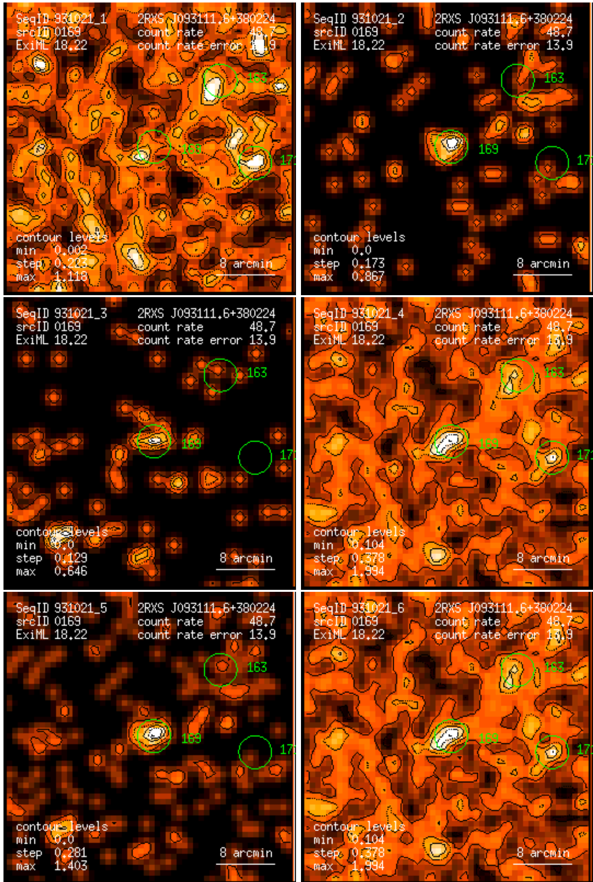
Figure 169: RASS 931021: detection 0169: band rate images, Gaussian filter: (1) PSPC channels 11 – 41, (2) 52 – 90, (3) 91 – 201, (4) 11 – 235, (5) 52 – 201, (6) 11 – 201. Broad band rates in counts/ks. Band rate contour levels in counts/ks/arcmin 2 .
