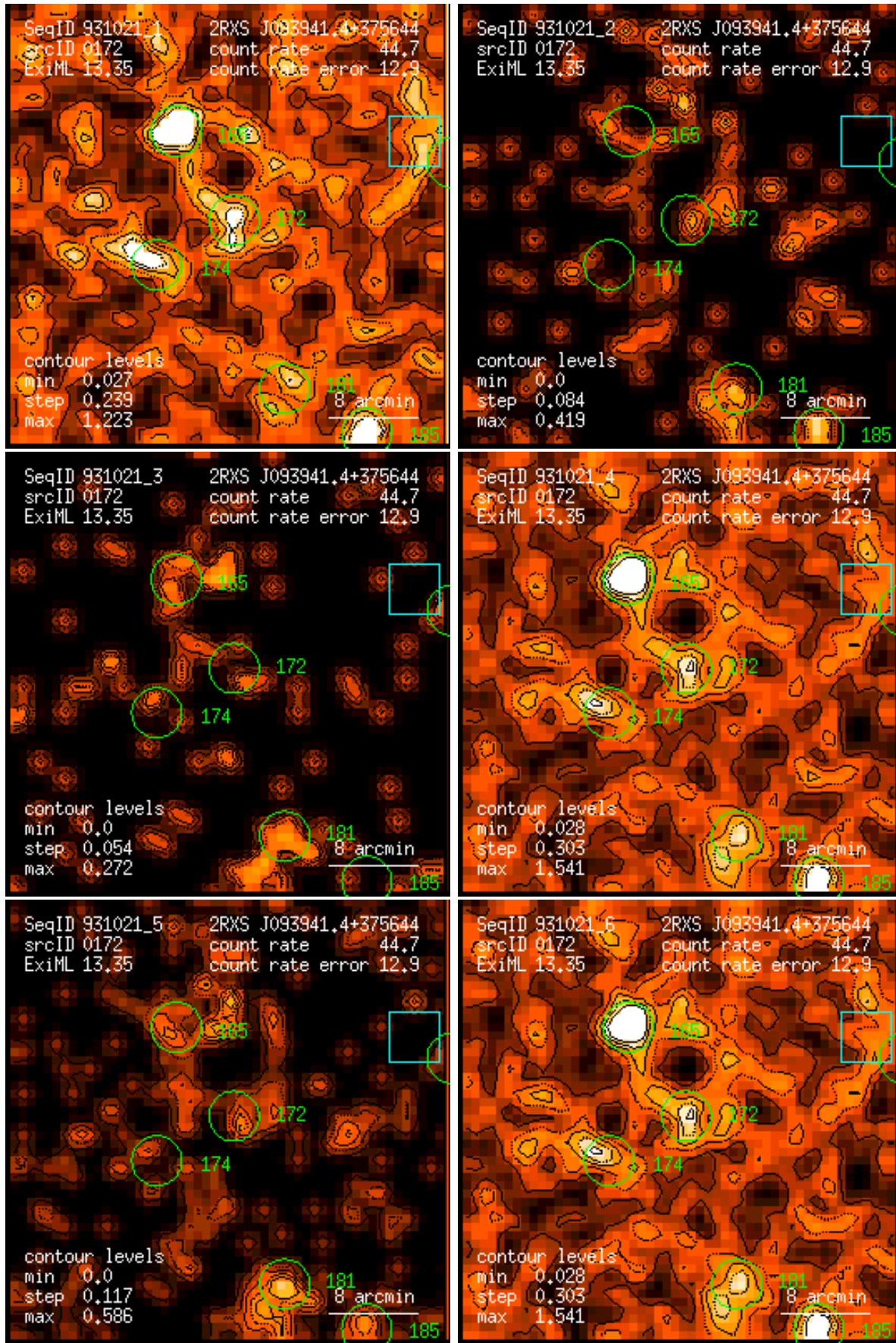
Figure 172: RASS 931021: detection 0172: band rate images, Gaussian filter: (1) PSPC channels 11 – 41, (2) 52 – 90, (3) 91 – 201, (4) 11 – 235, (5) 52 – 201, (6) 11 – 201. Broad band rates in counts/ks. Band rate contour levels in counts/ks/arcmin 2 .
