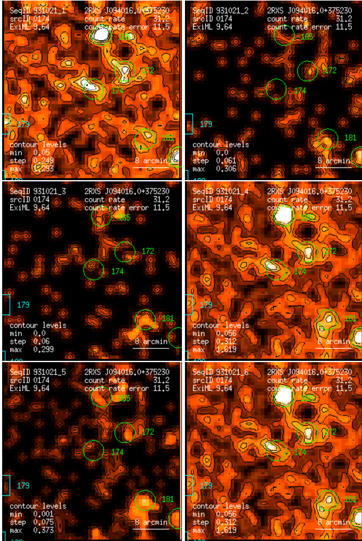
Figure 174: RASS 931021: detection 0174: band rate images, Gaussian filter: (1) PSPC channels 11 – 41, (2) 52 – 90, (3) 91 – 201, (4) 11 – 235, (5) 52 – 201, (6) 11 – 201. Broad band rates in counts/ks. Band rate contour levels in counts/ks/arcmin 2 .
