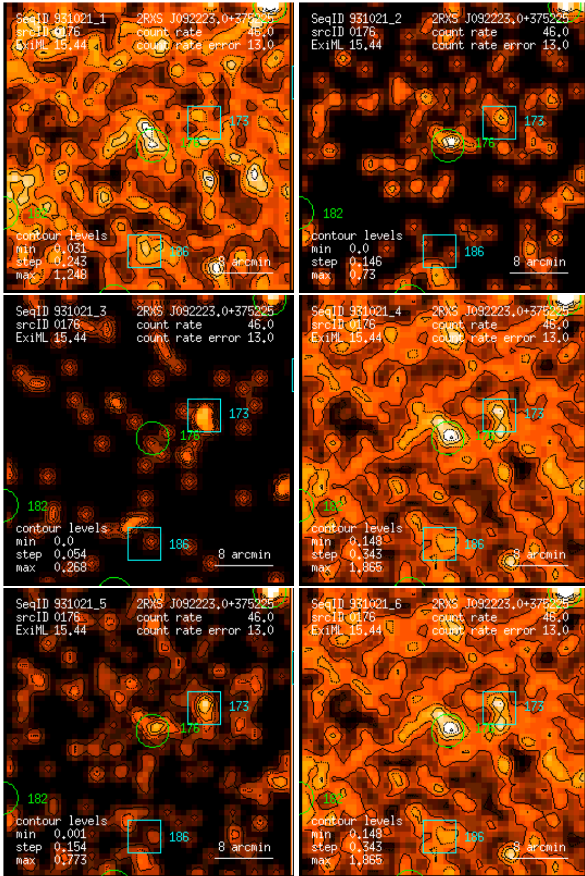
Figure 176: RASS 931021: detection 0176: band rate images, Gaussian filter: (1) PSPC channels 11 – 41, (2) 52 – 90, (3) 91 – 201, (4) 11 – 235, (5) 52 – 201, (6) 11 – 201. Broad band rates in counts/ks. Band rate contour levels in counts/ks/arcmin 2 .
