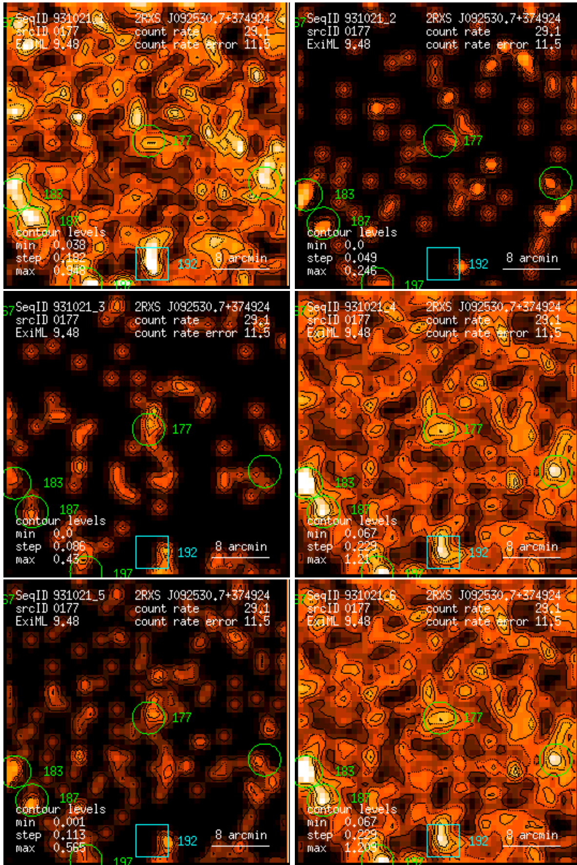
Figure 177: RASS 931021: detection 0177: band rate images, Gaussian filter: (1) PSPC channels 11 – 41, (2) 52 – 90, (3) 91 – 201, (4) 11 – 235, (5) 52 – 201, (6) 11 – 201. Broad band rates in counts/ks. Band rate contour levels in counts/ks/arcmin 2 .
