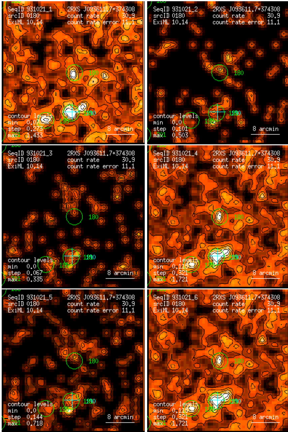
Figure 180: RASS 931021: detection 0180: band rate images, Gaussian filter: (1) PSPC channels 11 – 41, (2) 52 – 90, (3) 91 – 201, (4) 11 – 235, (5) 52 – 201, (6) 11 – 201. Broad band rates in counts/ks. Band rate contour levels in counts/ks/arcmin 2 .
