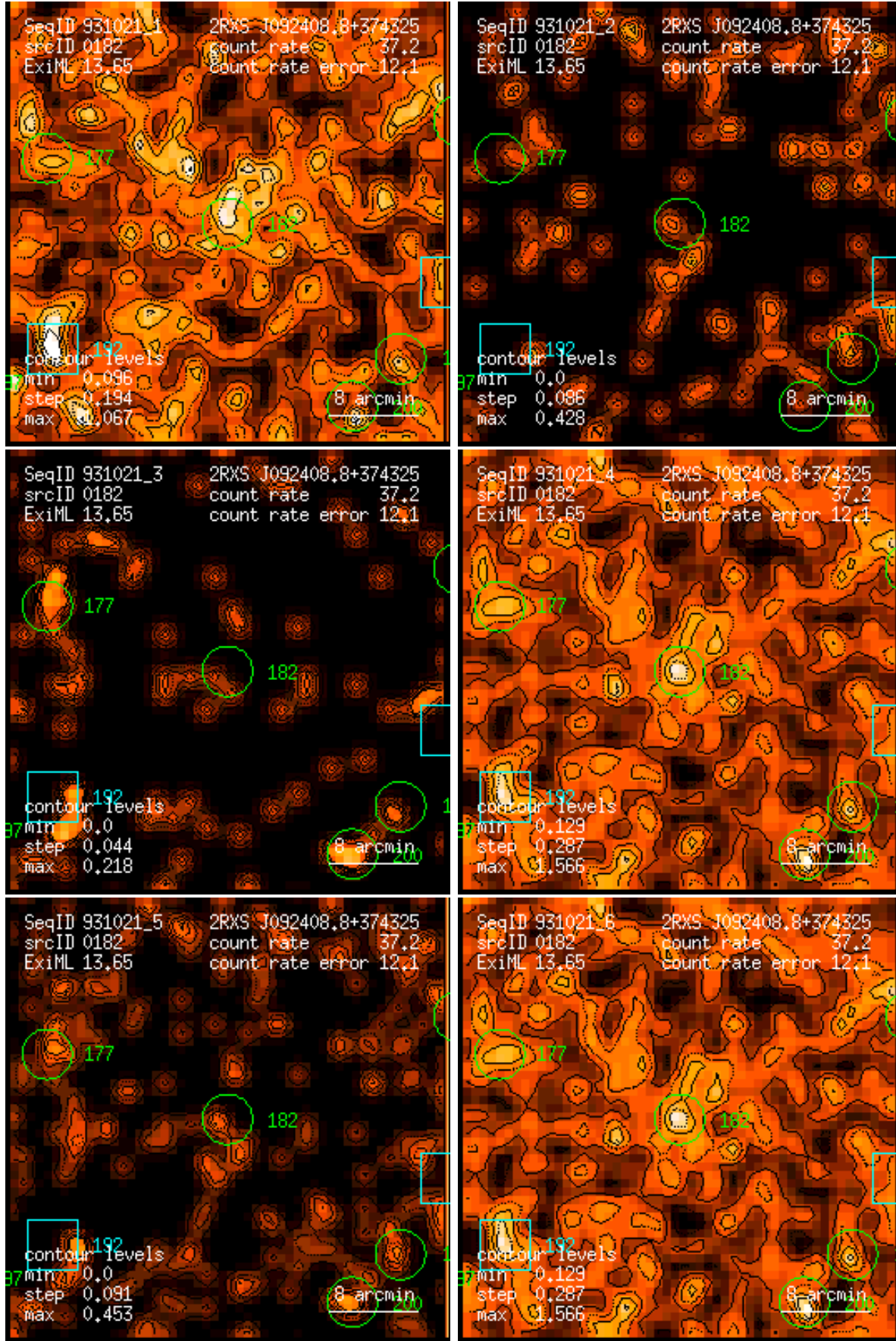
Figure 182: RASS 931021: detection 0182: band rate images, Gaussian filter: (1) PSPC channels 11 – 41, (2) 52 – 90, (3) 91 – 201, (4) 11 – 235, (5) 52 – 201, (6) 11 – 201. Broad band rates in counts/ks. Band rate contour levels in counts/ks/arcmin 2 .
