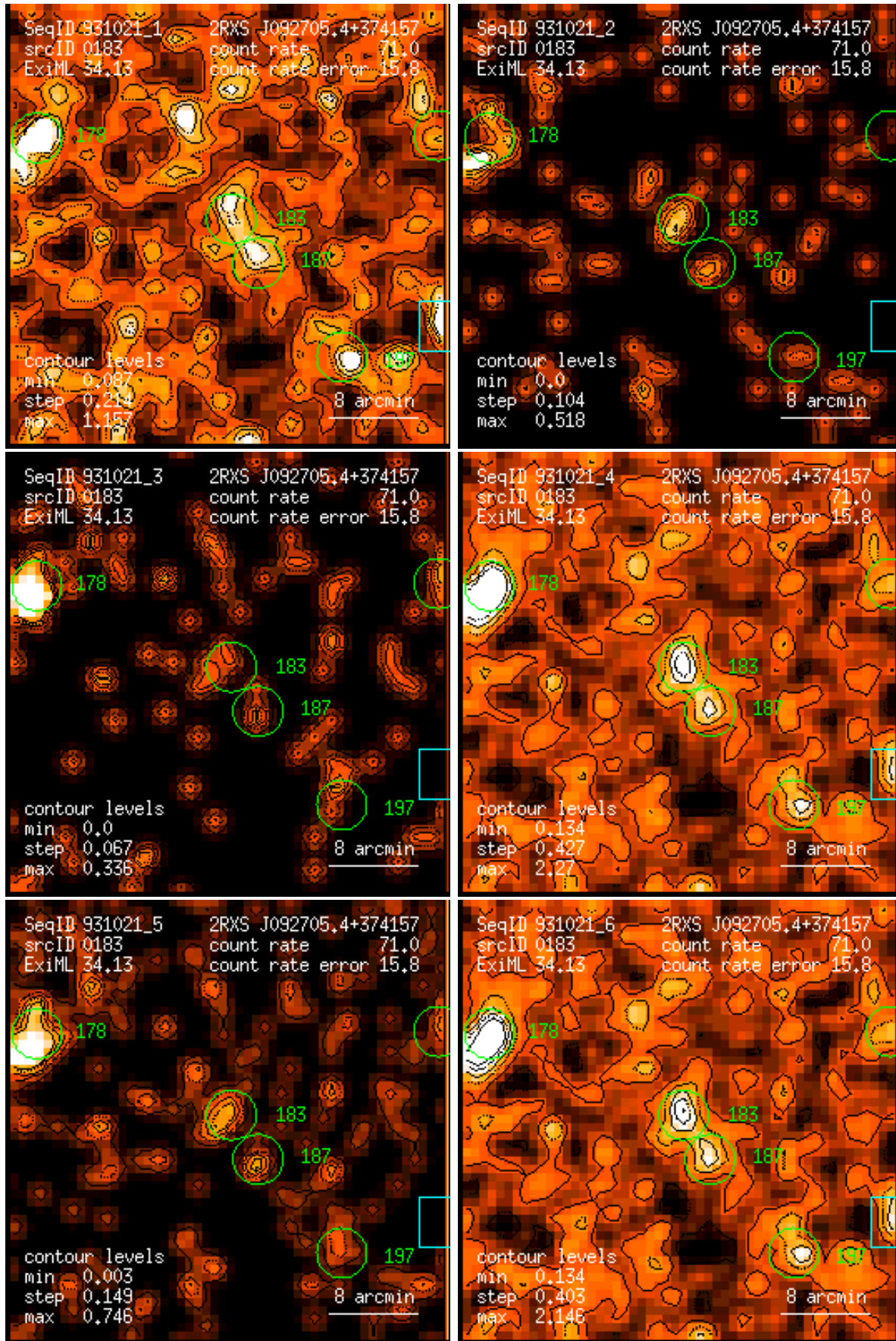
Figure 183: RASS 931021: detection 0183: band rate images, Gaussian filter: (1) PSPC channels 11 – 41, (2) 52 – 90, (3) 91 – 201, (4) 11 – 235, (5) 52 – 201, (6) 11 – 201. Broad band rates in counts/ks. Band rate contour levels in counts/ks/arcmin 2 .
