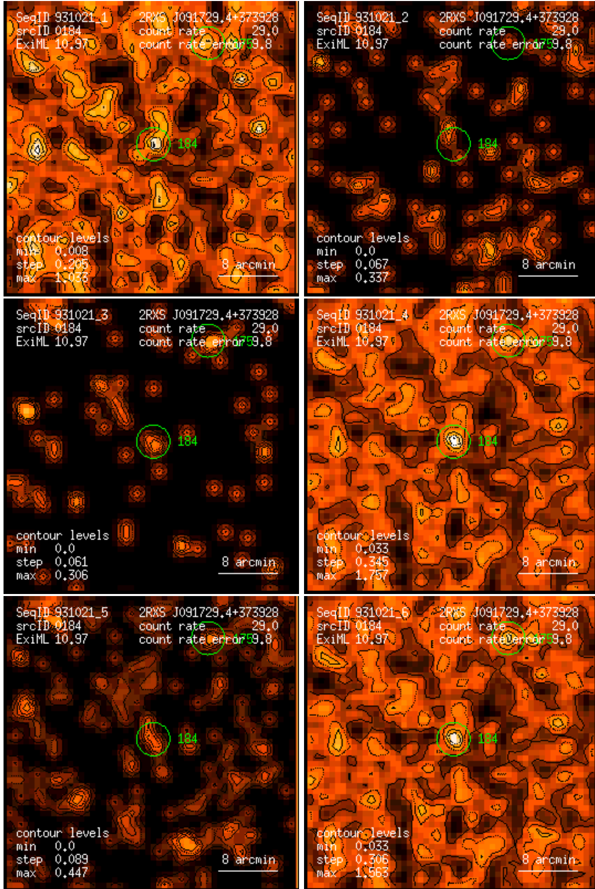
Figure 184: RASS 931021: detection 0184: band rate images, Gaussian filter: (1) PSPC channels 11 – 41, (2) 52 – 90, (3) 91 – 201, (4) 11 – 235, (5) 52 – 201, (6) 11 – 201. Broad band rates in counts/ks. Band rate contour levels in counts/ks/arcmin 2 .
