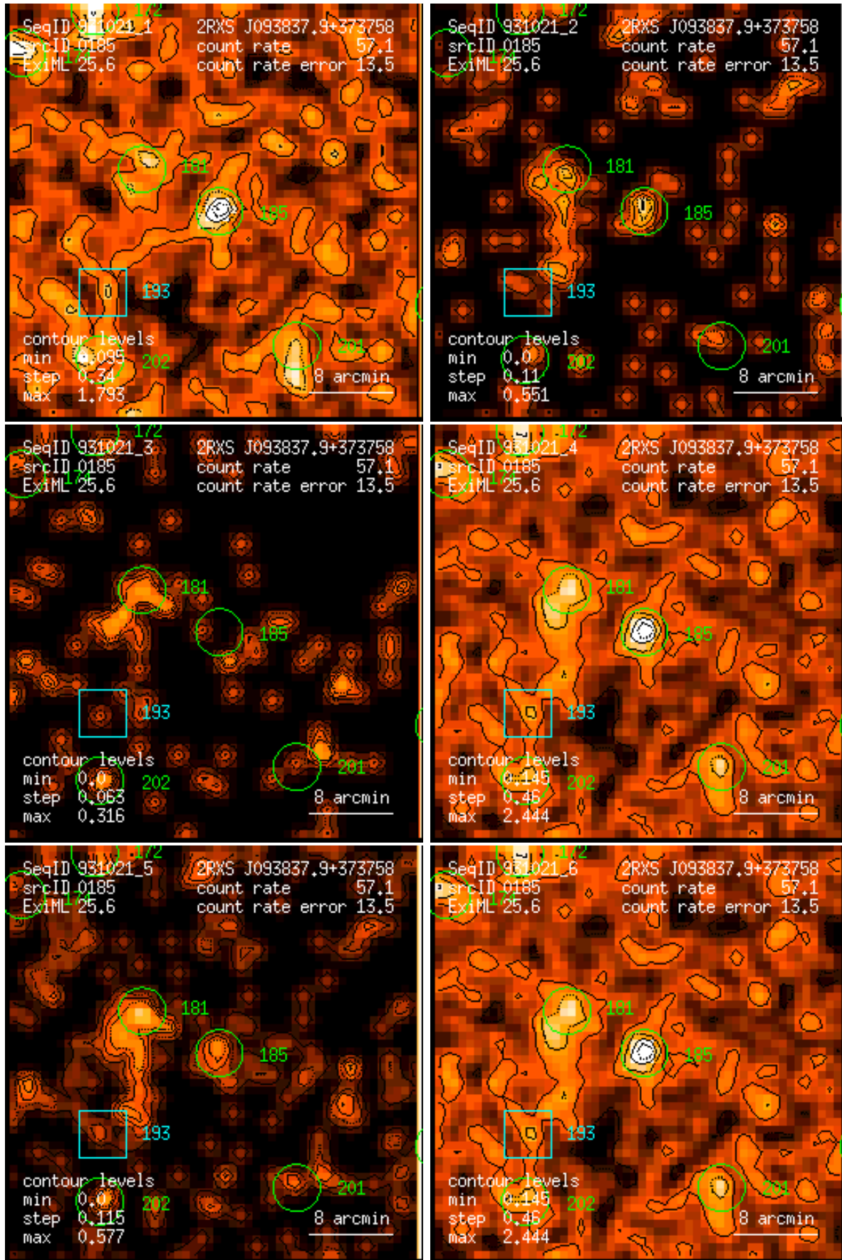
Figure 185: RASS 931021: detection 0185: band rate images, Gaussian filter: (1) PSPC channels 11 – 41, (2) 52 – 90, (3) 91 – 201, (4) 11 – 235, (5) 52 – 201, (6) 11 – 201. Broad band rates in counts/ks. Band rate contour levels in counts/ks/arcmin 2 .
