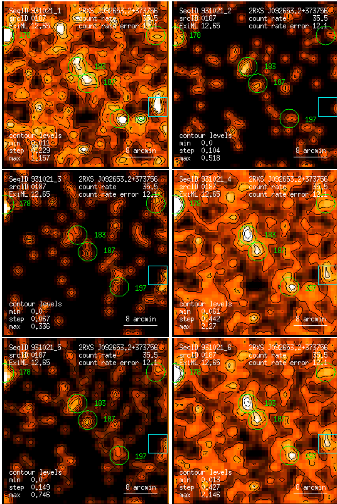
Figure 187: RASS 931021: detection 0187: band rate images, Gaussian filter: (1) PSPC channels 11 – 41, (2) 52 – 90, (3) 91 – 201, (4) 11 – 235, (5) 52 – 201, (6) 11 – 201. Broad band rates in counts/ks. Band rate contour levels in counts/ks/arcmin 2 .
