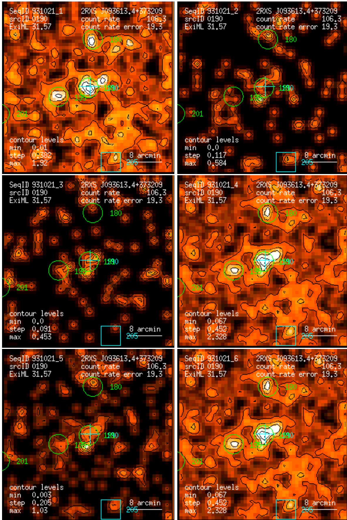
Figure 190: RASS 931021: detection 0190: band rate images, Gaussian filter: (1) PSPC channels 11 – 41, (2) 52 – 90, (3) 91 – 201, (4) 11 – 235, (5) 52 – 201, (6) 11 – 201. Broad band rates in counts/ks. Band rate contour levels in counts/ks/arcmin 2 .
