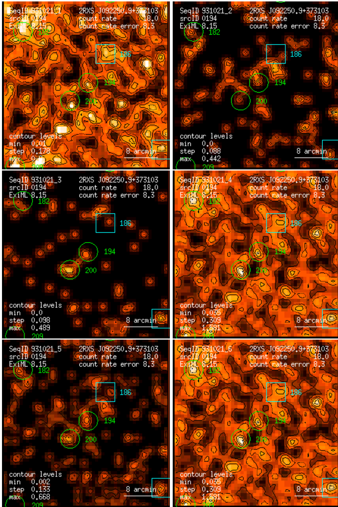
Figure 194: RASS 931021: detection 0194: band rate images, Gaussian filter: (1) PSPC channels 11 – 41, (2) 52 – 90, (3) 91 – 201, (4) 11 – 235, (5) 52 – 201, (6) 11 – 201. Broad band rates in counts/ks. Band rate contour levels in counts/ks/arcmin 2 .
