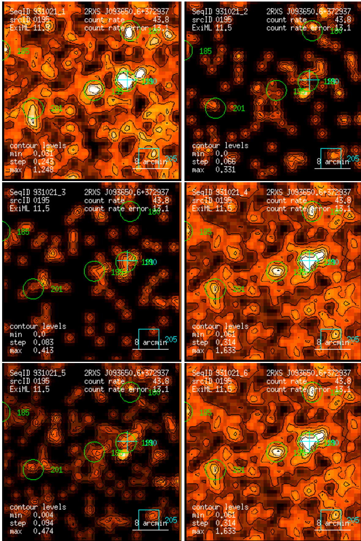
Figure 195: RASS 931021: detection 0195: band rate images, Gaussian filter: (1) PSPC channels 11 – 41, (2) 52 – 90, (3) 91 – 201, (4) 11 – 235, (5) 52 – 201, (6) 11 – 201. Broad band rates in counts/ks. Band rate contour levels in counts/ks/arcmin 2 .
