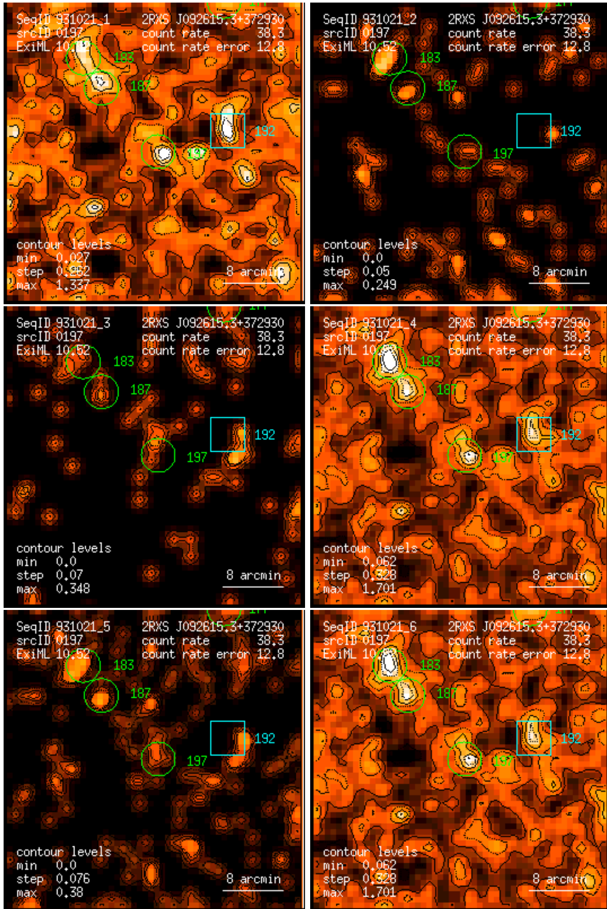
Figure 197: RASS 931021: detection 0197: band rate images, Gaussian filter: (1) PSPC channels 11 – 41, (2) 52 – 90, (3) 91 – 201, (4) 11 – 235, (5) 52 – 201, (6) 11 – 201. Broad band rates in counts/ks. Band rate contour levels in counts/ks/arcmin 2 .
